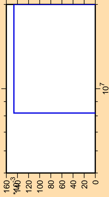
\Delta\sigma/\sigma vs. E for ^{223}\text{Ac} (mt 34)
