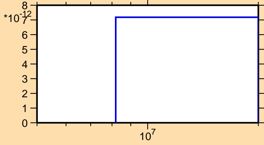
\sigma vs. E for ^{223}\text{Ac} (mt 45)
