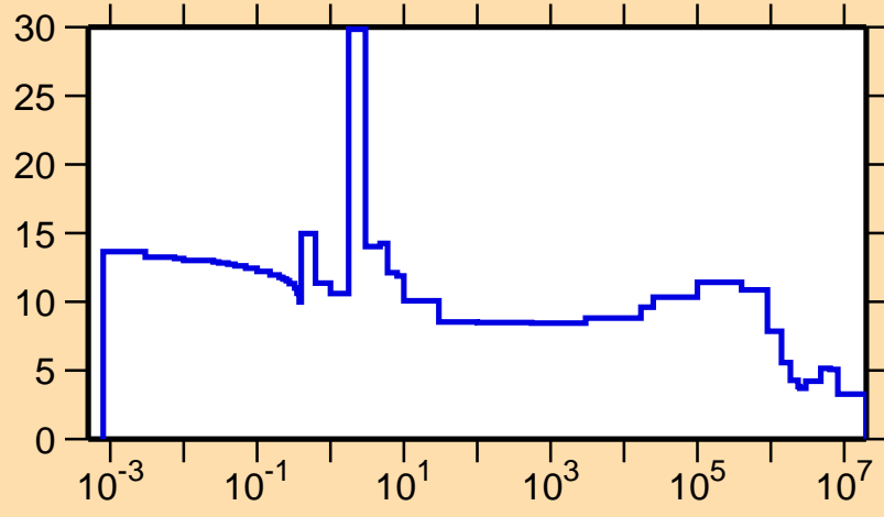
\sigma vs. E for ^{223}\text{Ac}(n,\text{el.})
