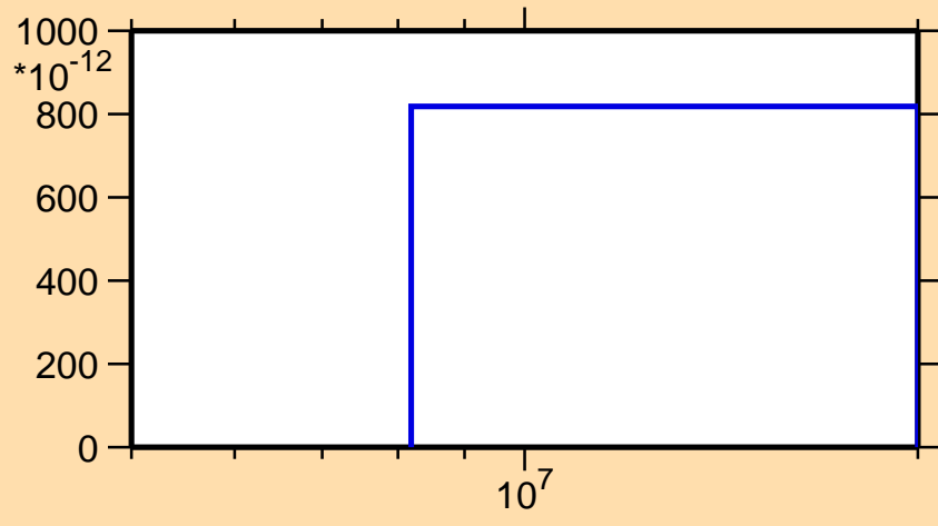
\sigma vs. E for ^{223}\text{Ac}(n,p\alpha)
