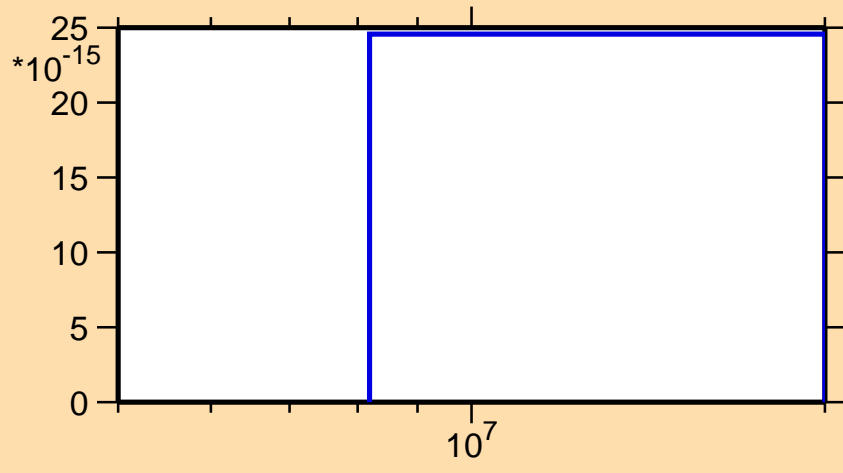
\sigma vs. E for ^{223}\text{Ac} (mt 34)
