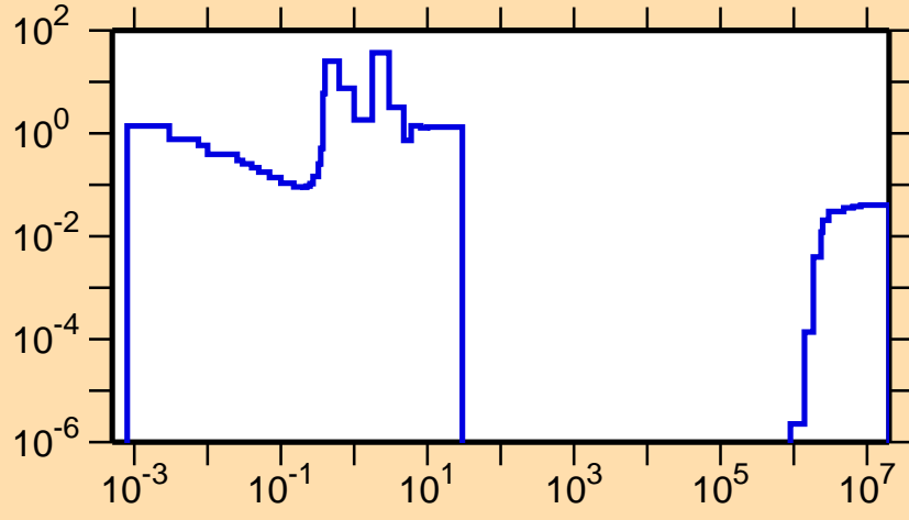
\sigma vs. E for ^{223}\text{Ac}(n,f)
