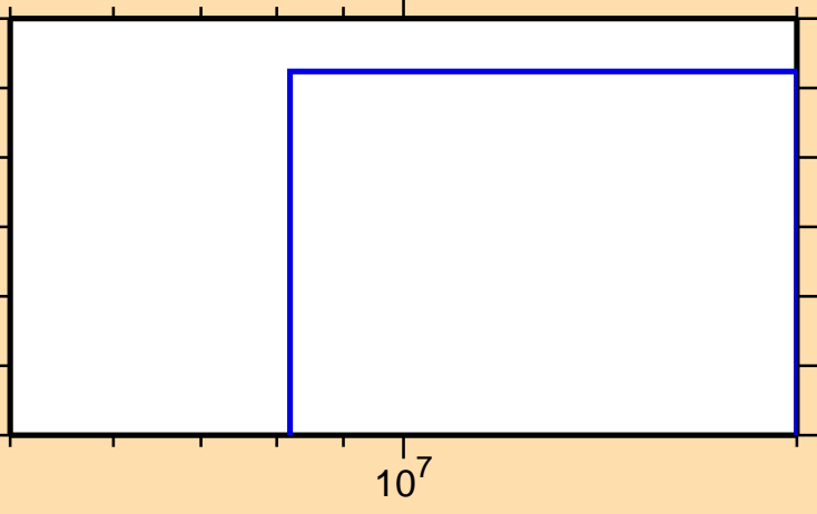
\sigma vs. E for ^{223}\text{Ac}(\text{mt117})
