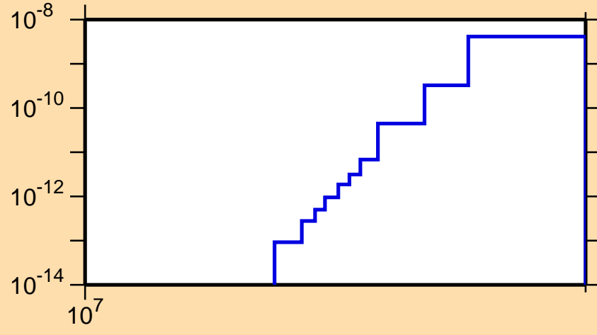
\sigma vs. E for ^{224}\text{Ac}(n,\text{He3})
