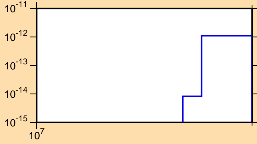
\sigma vs. E for ^{224}\text{Ac} (mt 34)
