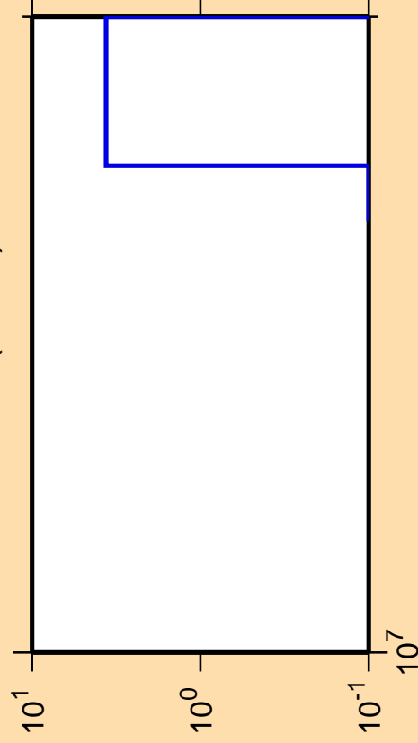
\Delta\sigma/\sigma vs. E for ^{224}\text{Ac} (mt 34)
