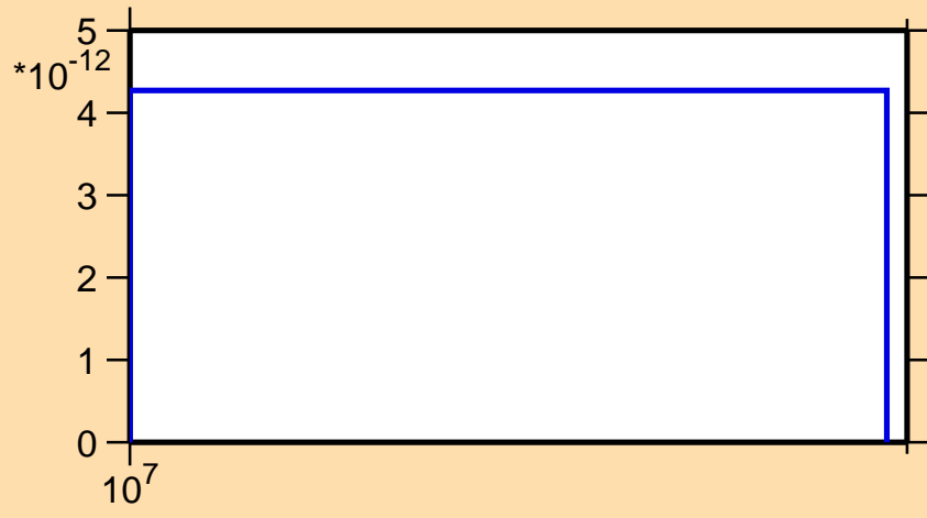
\sigma vs. E for ^{224}\text{Ac}(\text{mt117})
