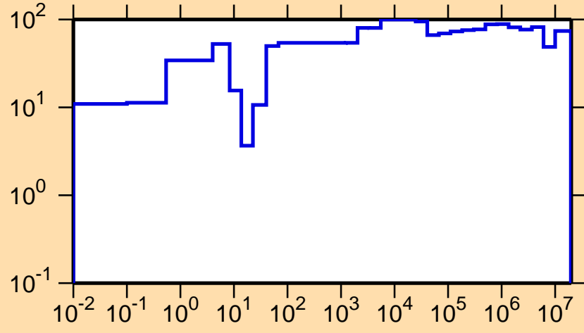
\Delta\sigma/\sigma vs. E for ^{224}\text{Ac}(n,\gamma)
