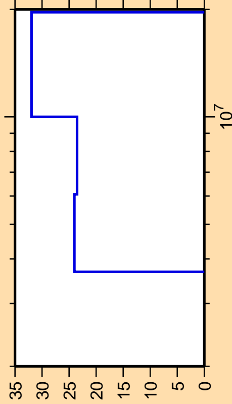
\Delta\sigma/\sigma vs. E for ^{224}\text{Ac}(n,n_1)
