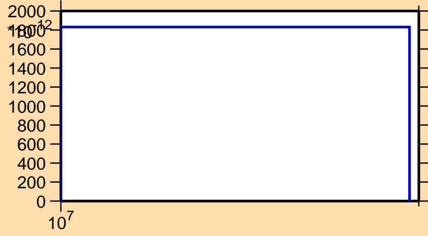
\sigma vs. E for ^{224}\text{Ac}(n,3n\alpha)
