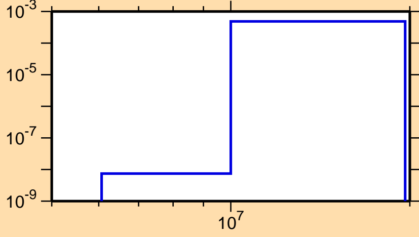
\sigma vs. E for ^{224}\text{Ac}(n,t)
