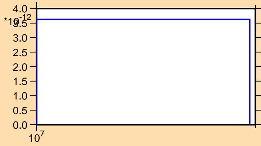
\sigma vs. E for ^{224}\text{Ac}(\text{mt } 45)
