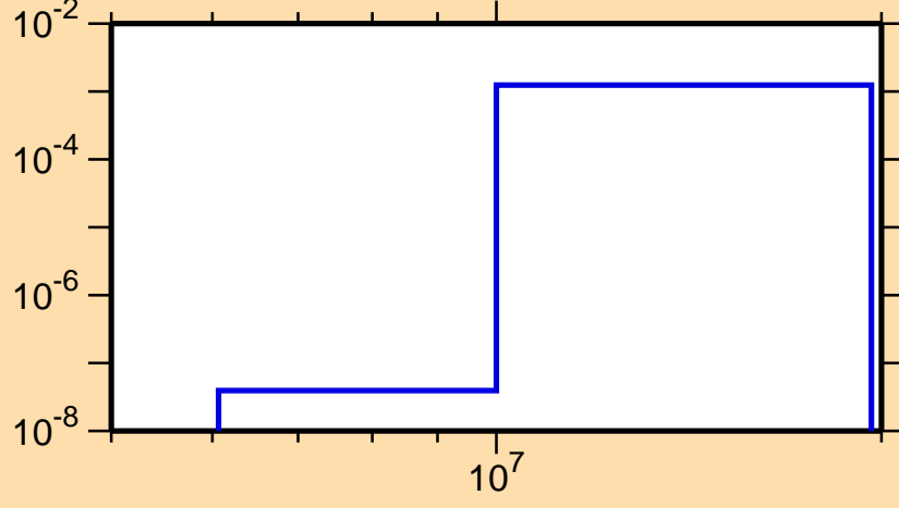
\sigma vs. E for ^{224}\text{Ac}(n,d)
