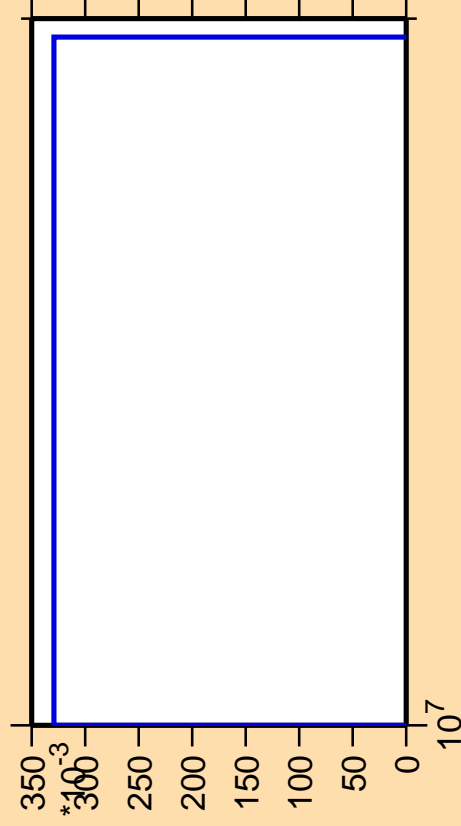
\Delta\sigma/\sigma vs. E for ^{224}\text{Ac} (mt 11)
