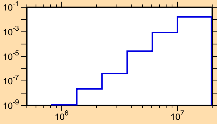
\sigma vs. E for ^{224}\text{Ac}(n,p)
