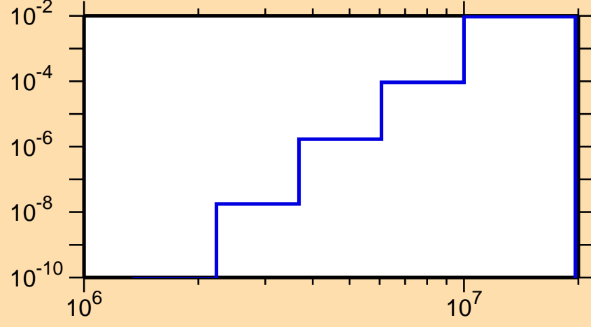
\sigma vs. E for ^{224}\text{Ac}(n,n\alpha)
