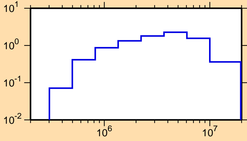
\sigma vs. E for ^{224}\text{Ac}(n,n\text{cont.})
