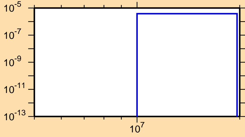
\sigma vs. E for ^{224}\text{Ac}(n,\text{nd})
