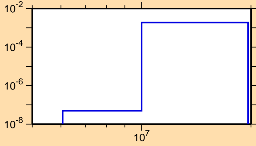
\sigma vs. E for ^{224}\text{Ac}(n,np)
