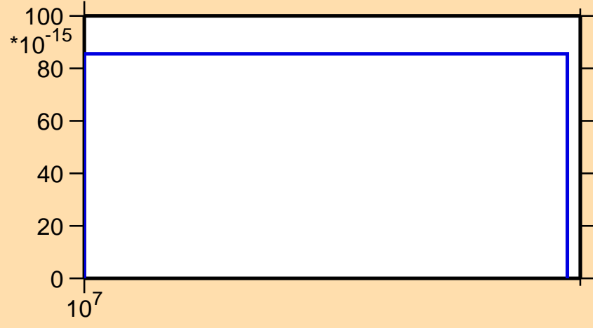
\sigma vs. E for ^{224}\text{Ac} (mt 11)
