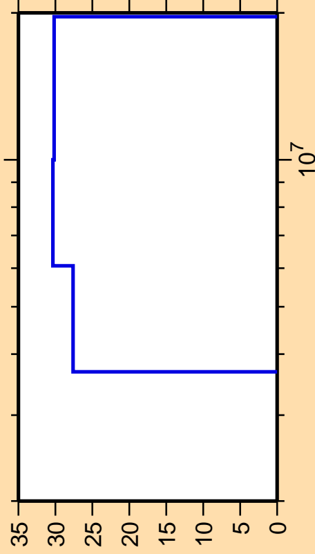
\Delta\sigma/\sigma vs. E for ^{224}\text{Ac}(n,n\text{cont.})
