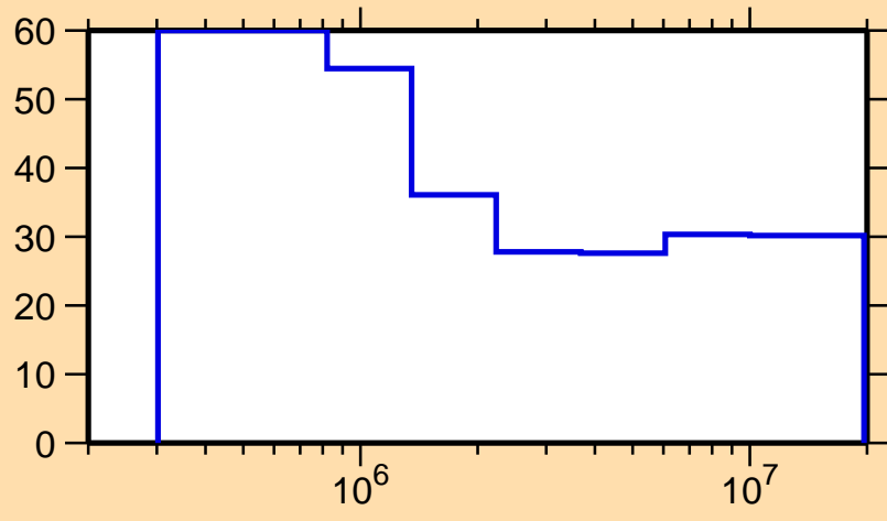
\Delta\sigma/\sigma vs. E for ^{224}\text{Ac}(n,n\text{cont.})
