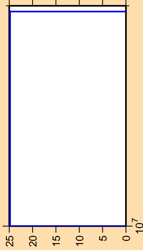
\Delta\sigma/\sigma vs. E for ^{224}\text{Ac}(\text{mt117})
