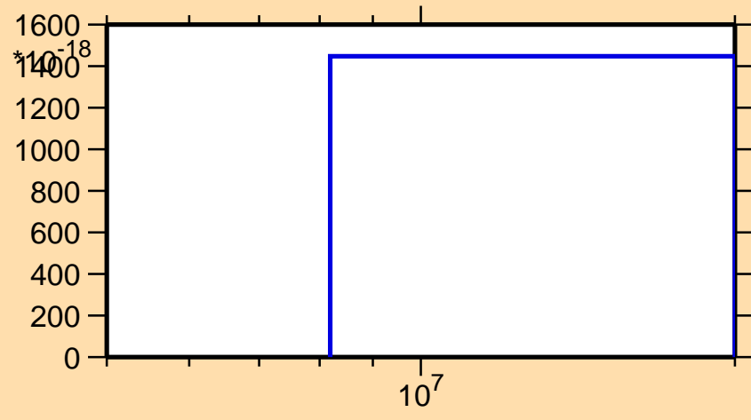
\sigma vs. E for ^{224}\text{Ac}(\text{mt } 42)
