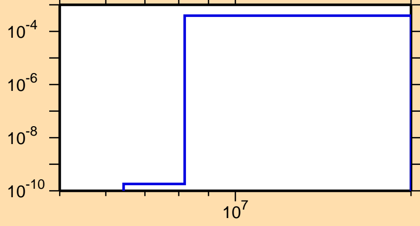
\sigma vs. E for ^{224}\text{Ac}(n,t)
