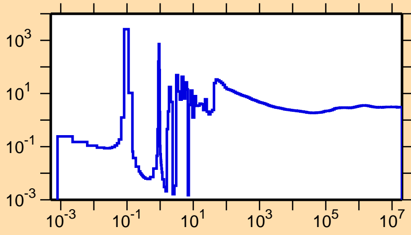
\sigma vs. E for ^{225}\text{Ac}(n,\text{nonel.})
