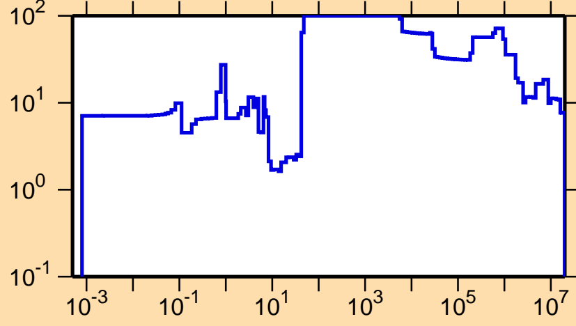
\Delta\sigma/\sigma vs. E for ^{225}\text{Ac}(n,el.)
