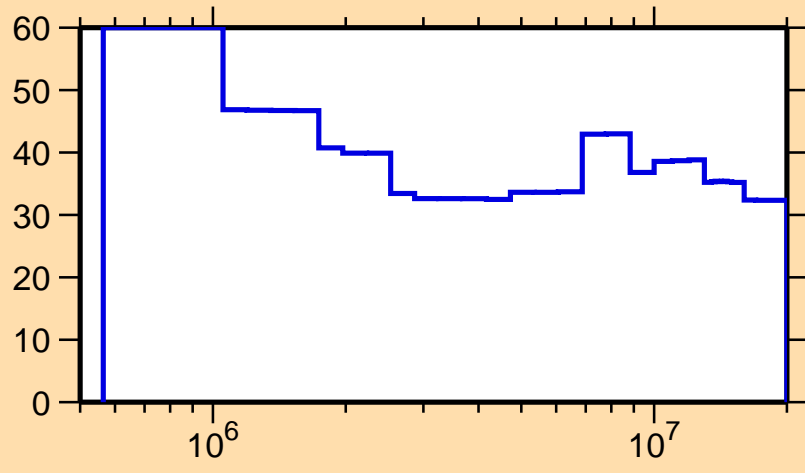
\Delta\sigma/\sigma vs. E for ^{225}\text{Ac}(n,n\text{cont.})
