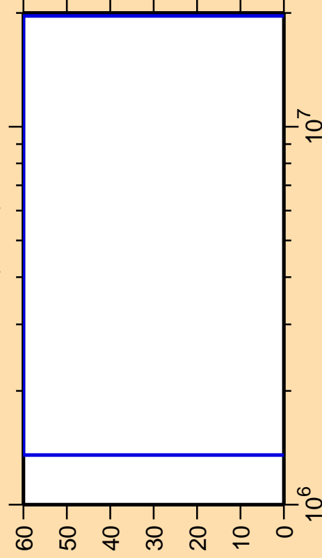
\Delta\sigma/\sigma vs. E for ^{225}\text{Ac}(n,n\alpha)
