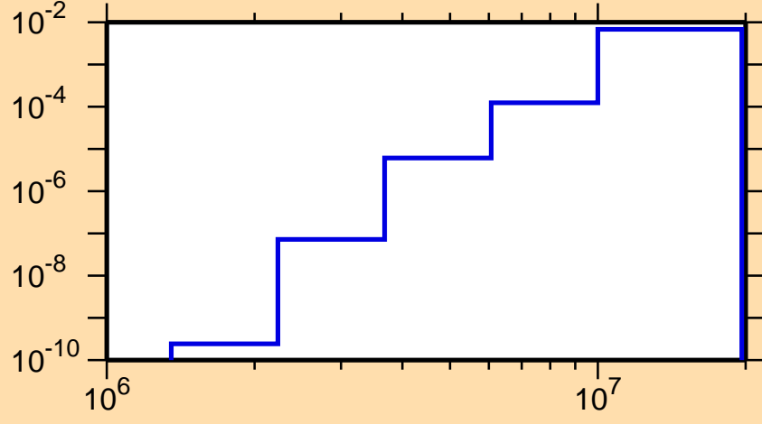
\sigma vs. E for ^{225}\text{Ac}(n,n\alpha)
