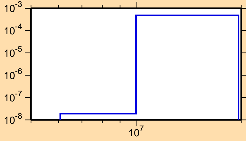
\sigma vs. E for ^{225}\text{Ac}(n,d)
