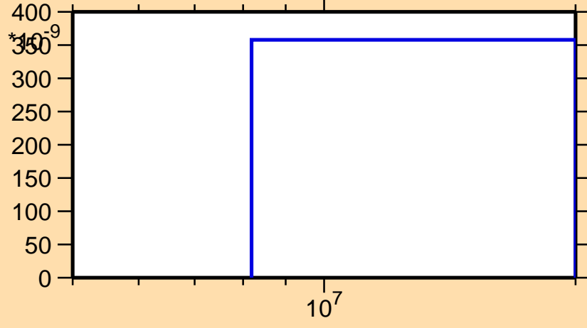
\sigma vs. E for ^{225}\text{Ac}(n,p\alpha)
