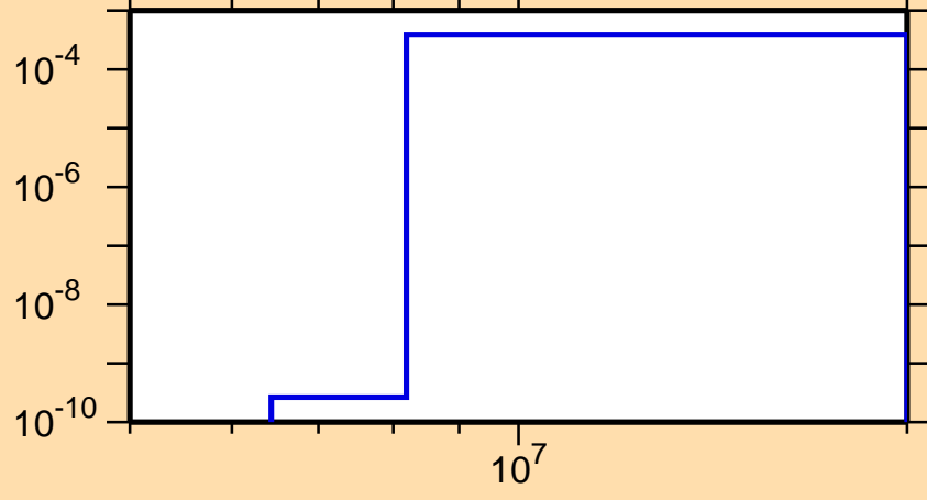
\sigma vs. E for ^{225}\text{Ac}(n,d)
