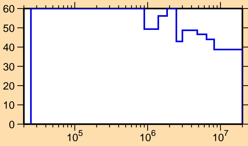
\Delta\sigma/\sigma vs. E for ^{225}\text{Ac}(n,n_1)
