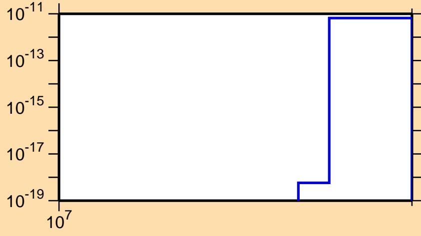
\sigma vs. E for ^{226}\text{Ac}(\text{mt } 11)
