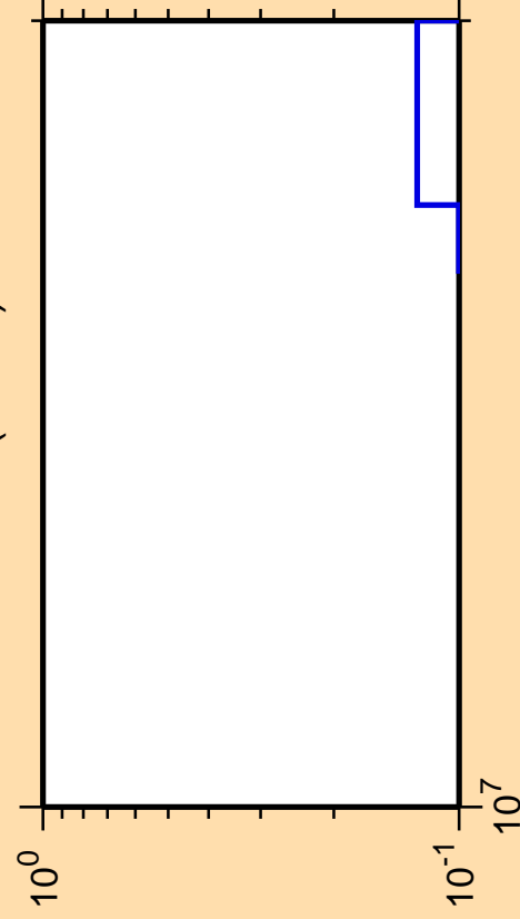
\Delta\sigma/\sigma vs. E for ^{226}\text{Ac}(\text{mt } 34)
