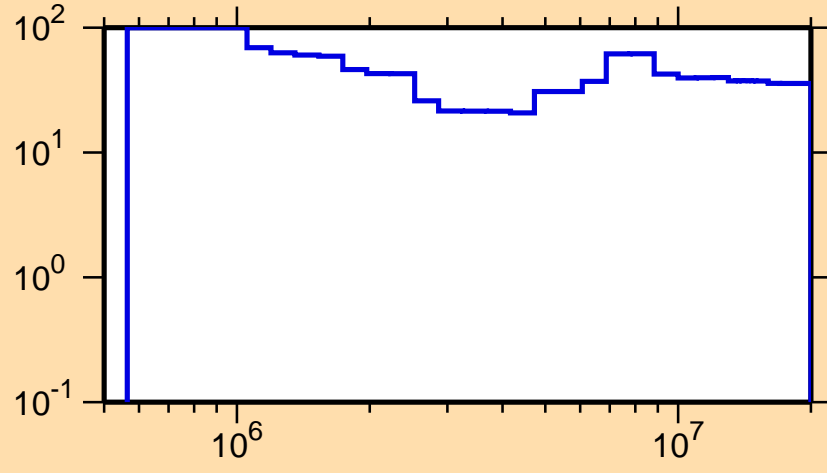
\Delta\sigma/\sigma vs. E for ^{226}\text{Ac}(n,n\text{cont.})
