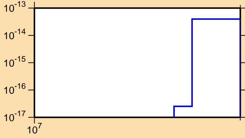
\sigma vs. E for ^{226}\text{Ac}(\text{mt } 34)
