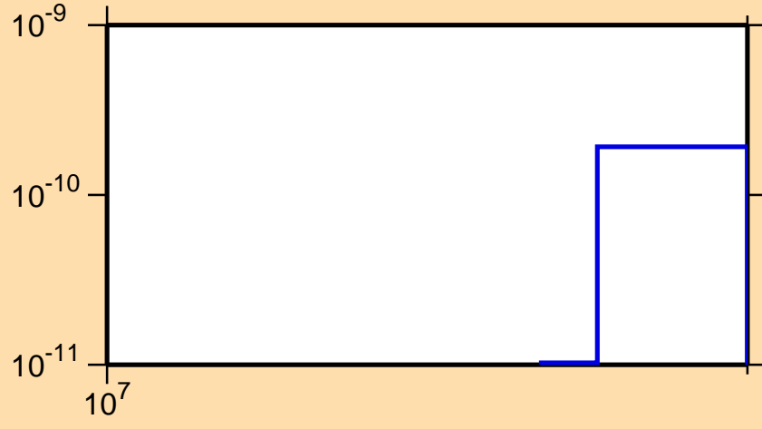
\sigma vs. E for ^{226}\text{Ac}(n,\text{He3})
