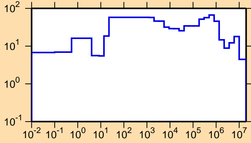
\Delta\sigma/\sigma vs. E for ^{226}\text{Ac}(n,el.)
