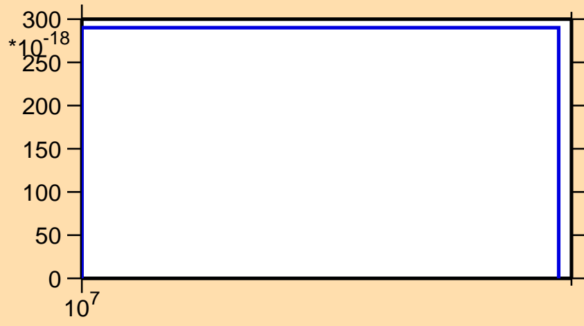
\sigma vs. E for ^{226}\text{Ac}(\text{mt } 34)
