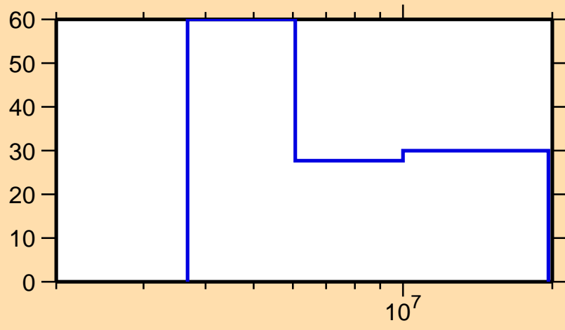
\Delta\sigma/\sigma vs. E for ^{226}\text{Ac}(n,2n)
