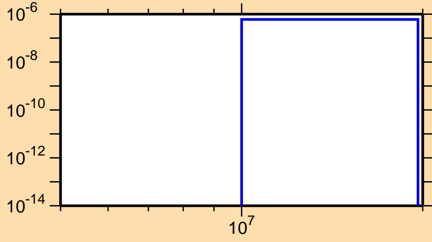
\sigma vs. E for ^{226}\text{Ac}(n,nt)
