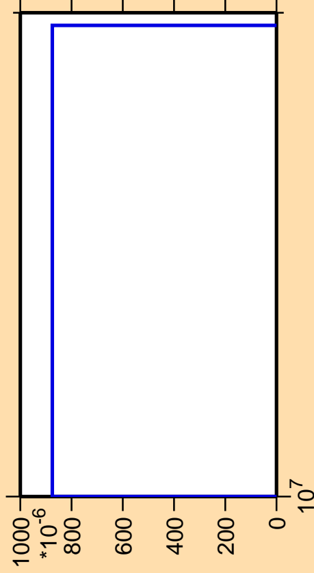
\Delta\sigma/\sigma vs. E for ^{226}\text{Ac}(\text{mt } 34)
