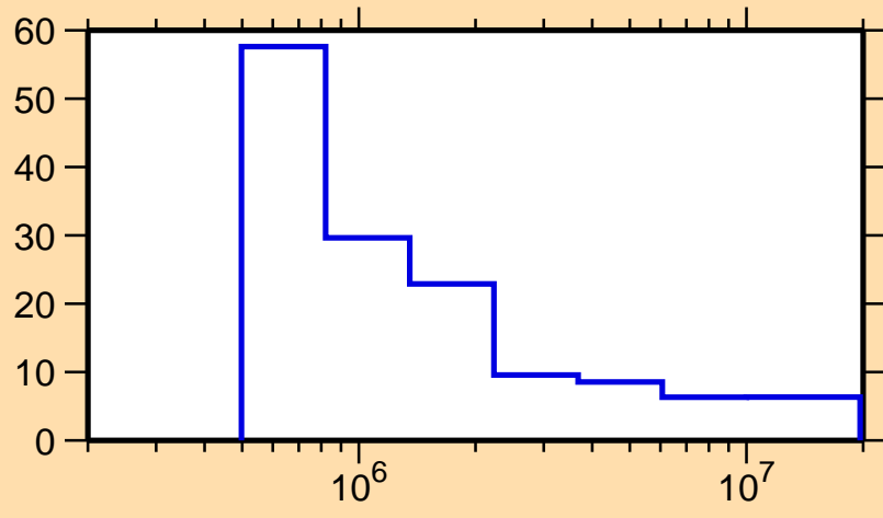
\Delta\sigma/\sigma vs. E for ^{226}\text{Ac}(n,\text{nonel.})
