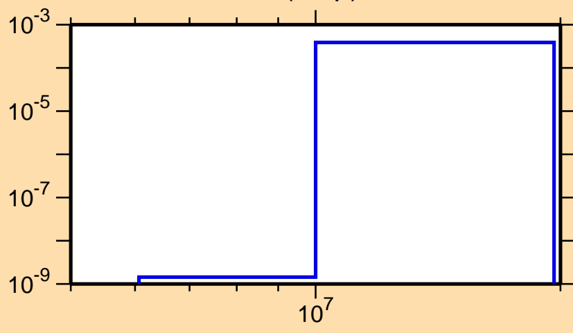
\sigma vs. E for ^{226}\text{Ac}(n,np)
