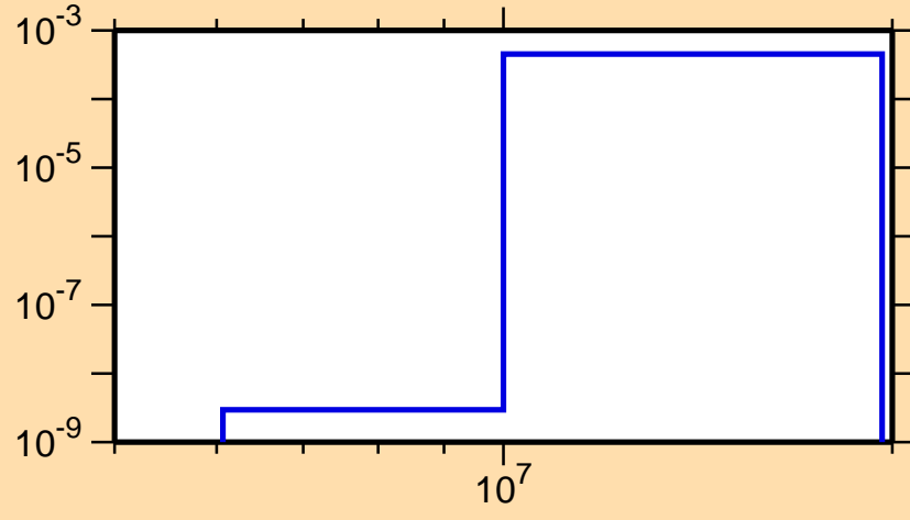
\sigma vs. E for ^{226}\text{Ac}(n,d)
