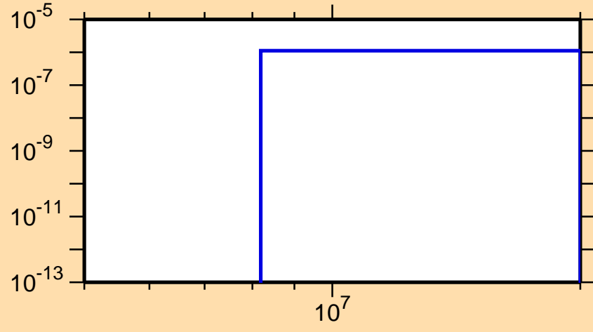
\sigma vs. E for ^{226}\text{Ac}(n,\text{nd})
