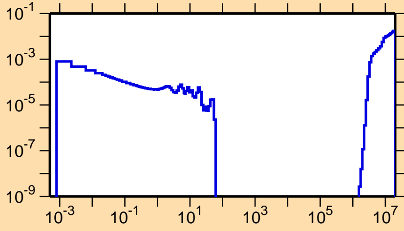
\sigma vs. E for ^{227}\text{Ac}(n,f)
