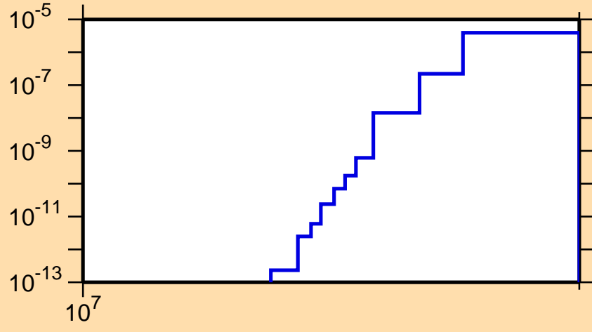
\sigma vs. E for ^{227}\text{Ac}(n,\text{nd})
