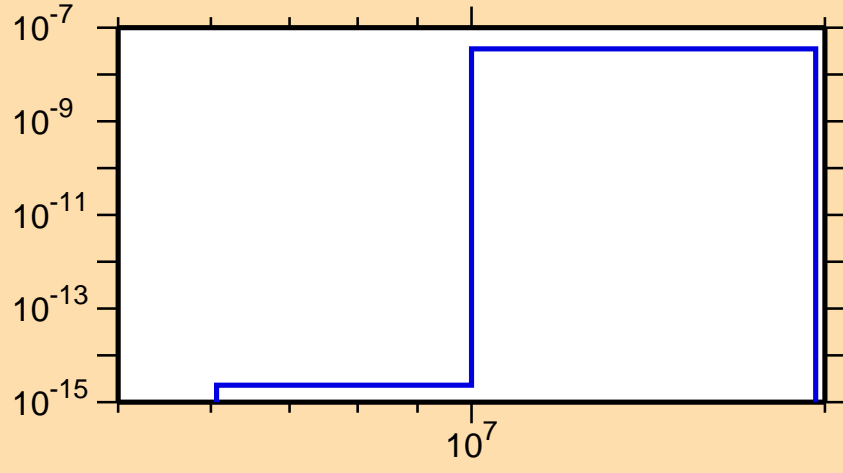
\sigma vs. E for ^{227}\text{Ac}(n,2n\alpha)
