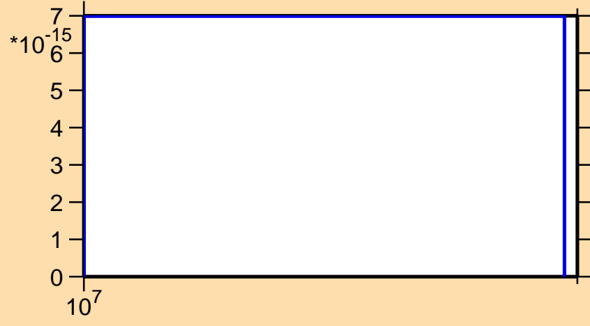
\sigma vs. E for ^{227}\text{Ac} (mt 11)
