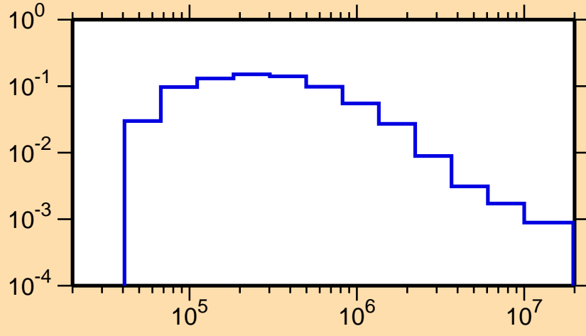
\sigma vs. E for ^{227}\text{Ac}(n,n_3)
