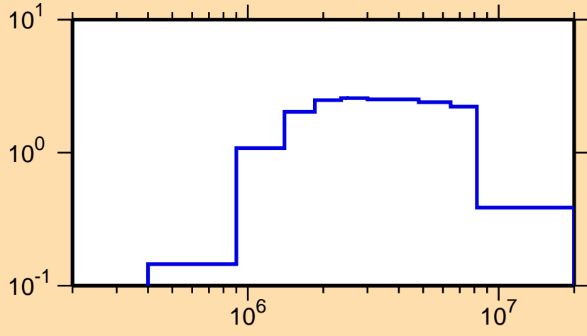
\sigma vs. E for ^{227}\text{Ac}(n,n\text{cont.})
