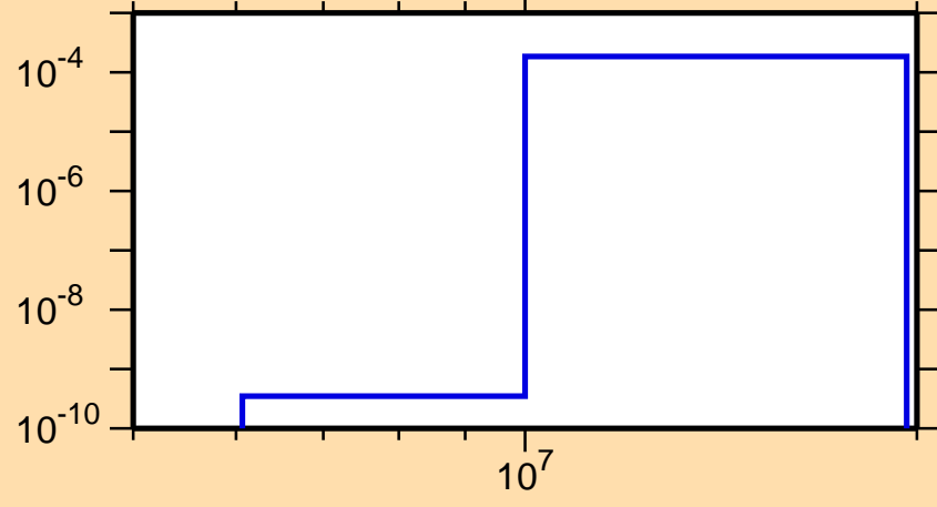
\sigma vs. E for ^{228}\text{Ac}(n,np)
