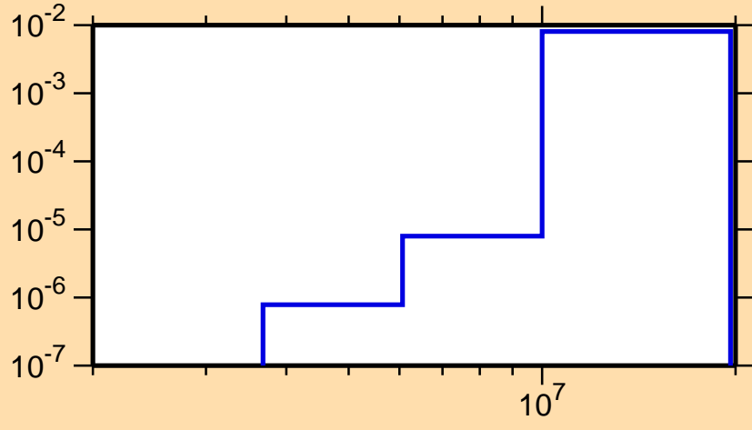
\sigma vs. E for ^{228}\text{Ac}(n,n\alpha)
