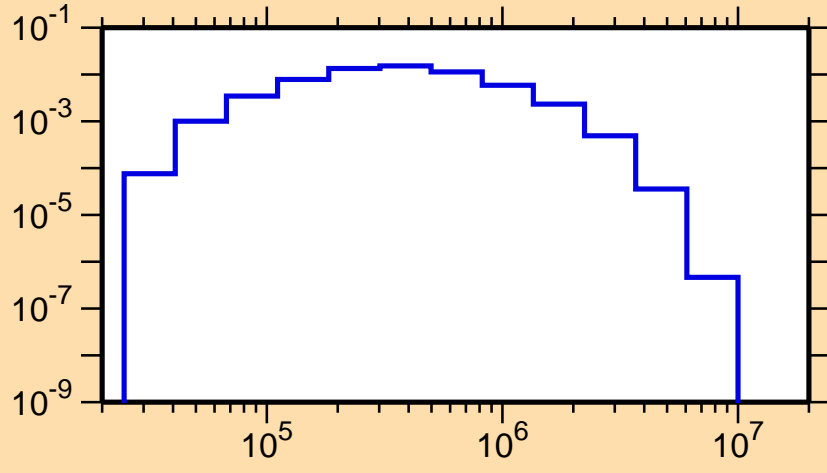
\sigma vs. E for ^{228}\text{Ac}(n,n_4)
