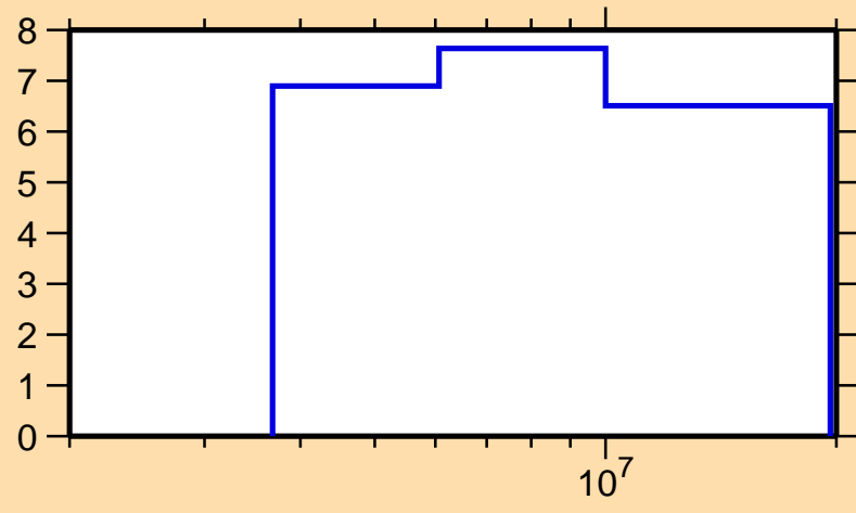
\Delta\sigma/\sigma vs. E for ^{228}\text{Ac}(n,\text{el.})
