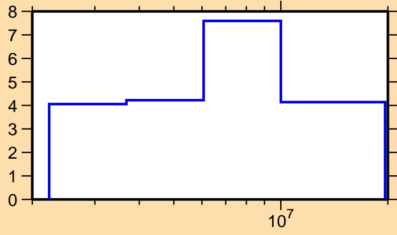
\Delta\sigma/\sigma vs. E for ^{228}\text{Ac}(n,\text{tot.})
