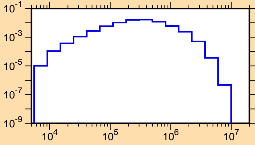
\sigma vs. E for ^{228}\text{Ac}(n,n_2)
