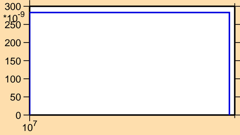
\sigma vs. E for ^{228}\text{Ac}(n,nt)
