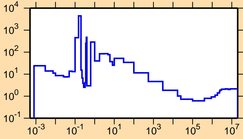
\sigma vs. E for ^{228}\text{Ac}(n,\text{nonel.})
