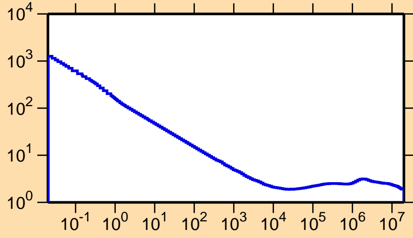
\sigma vs. E for ^{229}\text{Ac}(n,\alpha)
