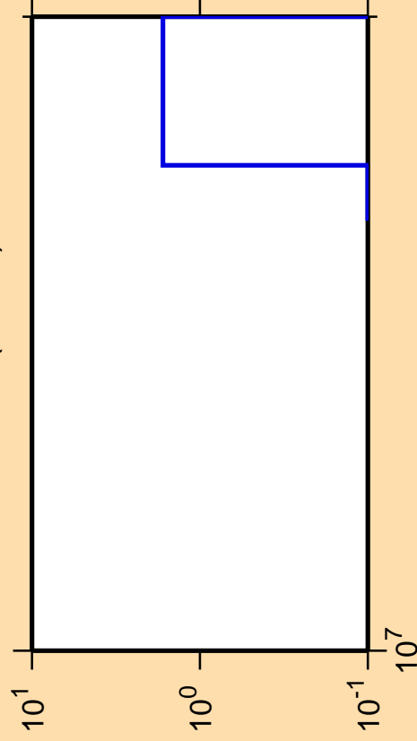
\Delta\sigma/\sigma vs. E for ^{229}\text{Ac} (mt 11)
