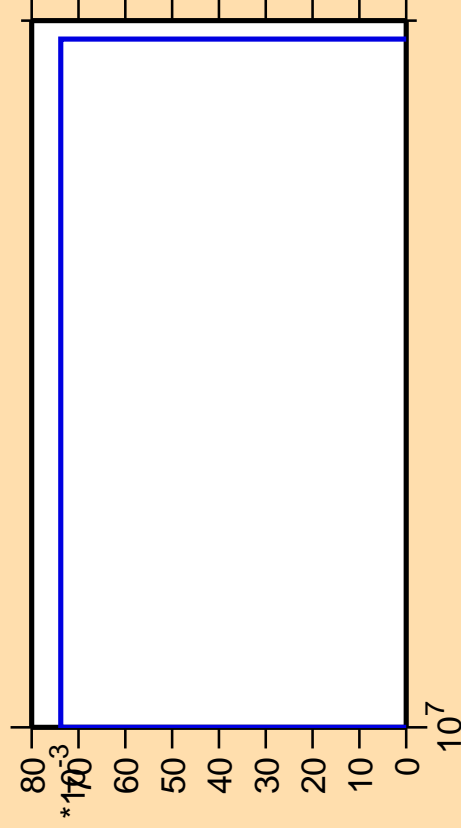
\Delta\sigma/\sigma vs. E for ^{229}\text{Ac}(n,3n\alpha)
