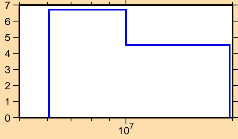
\Delta\sigma/\sigma vs. E for ^{229}\text{Ac}(n,\text{nonel.})
