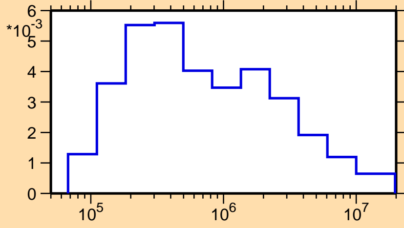
\sigma vs. E for ^{229}\text{Ac}(n,n_4)
