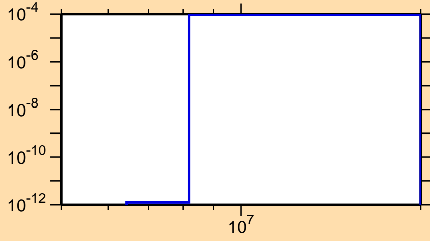
\sigma vs. E for ^{229}\text{Ac}(n,d)
