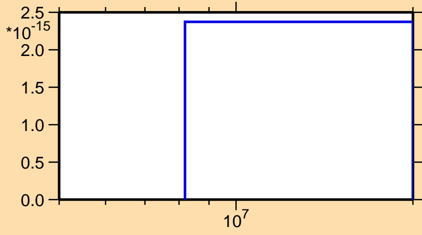
\sigma vs. E for ^{229}\text{Ac} (mt 11)
