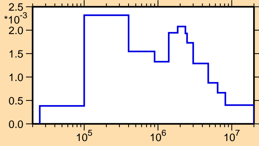
\sigma vs. E for ^{229}\text{Ac}(n,n_3)
