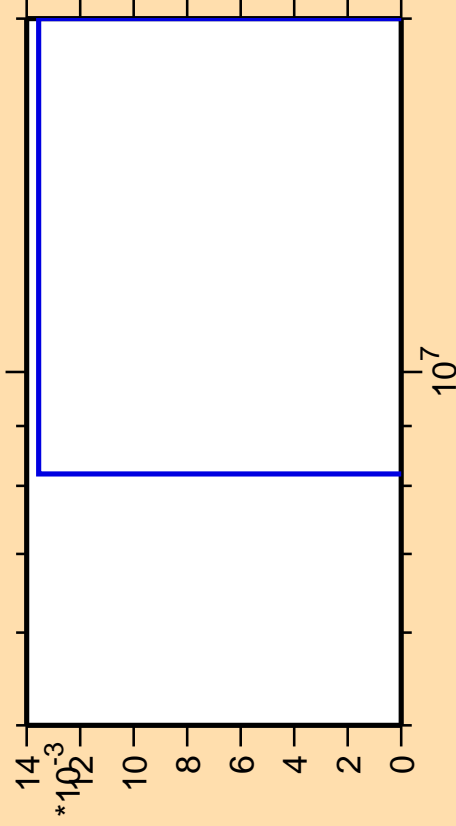
\Delta\sigma/\sigma vs. E for ^{229}\text{Ac} (mt 11)
