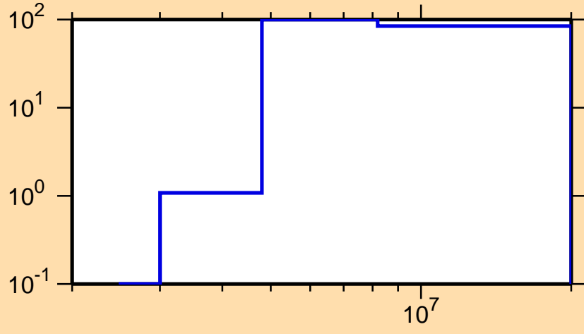
\Delta\sigma/\sigma vs. E for ^{229}\text{Ac}(n,p)
