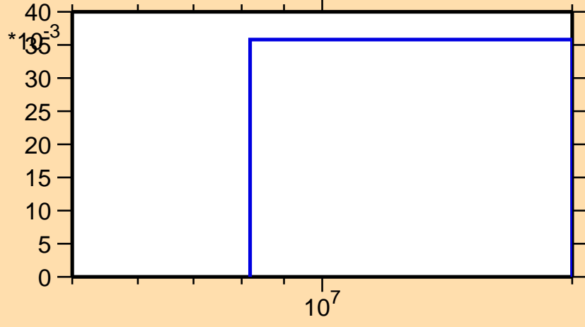
\sigma vs. E for ^{229}\text{Ac}(n,3n)
