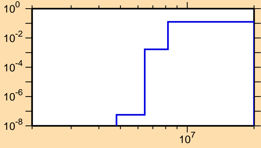
\sigma vs. E for ^{229}\text{Ac}(n,2n)
