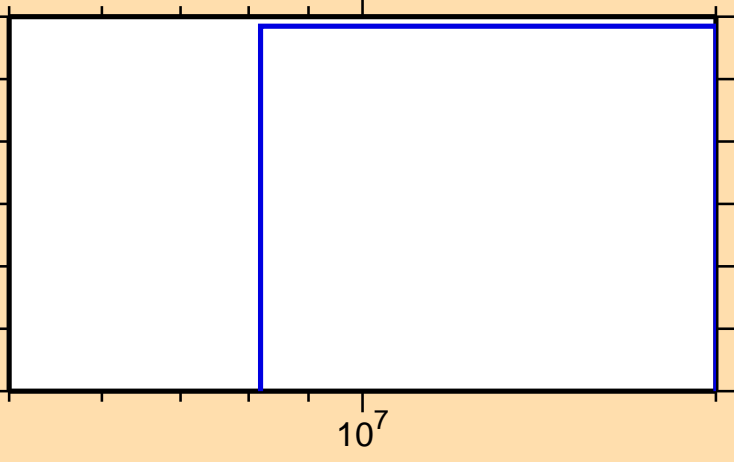
\sigma vs. E for ^{229}\text{Ac}(n,\text{nd})
