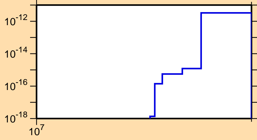
\sigma vs. E for ^{230}\text{Ac}(\text{mt } 11)
