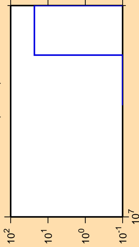
\Delta\sigma/\sigma vs. E for ^{230}\text{Ac}(\text{mt } 11)
