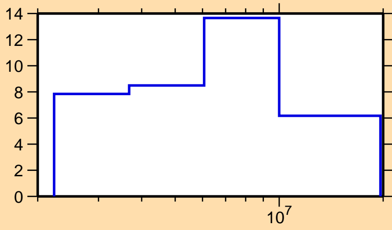
\Delta\sigma/\sigma vs. E for ^{230}\text{Ac}(n,\text{tot.})
