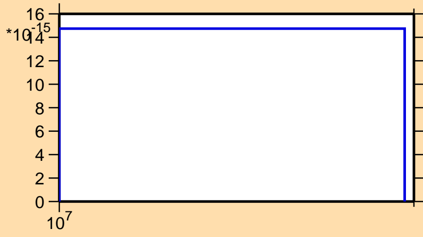
\sigma vs. E for ^{230}\text{Ac}(n,3n\alpha)
