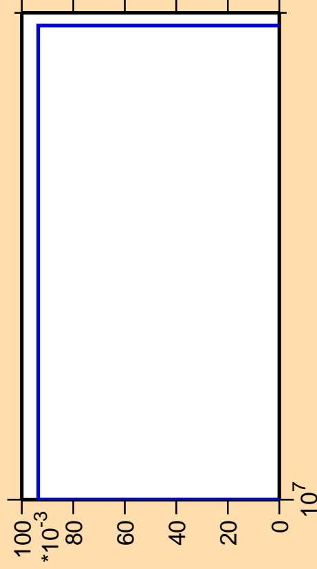
\Delta\sigma/\sigma vs. E for ^{230}\text{Ac}(n,3n\alpha)
