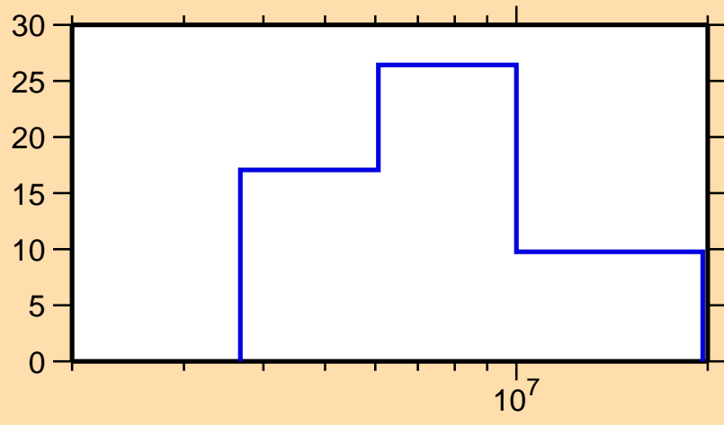
\Delta\sigma/\sigma vs. E for ^{230}\text{Ac}(n,\text{el.})
