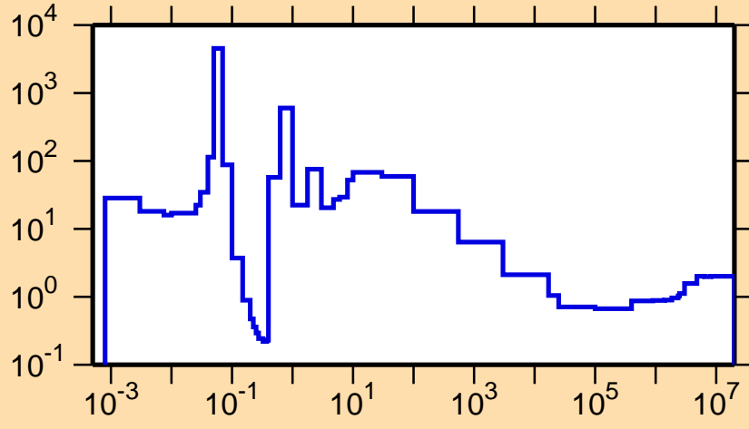
\sigma vs. E for ^{230}\text{Ac}(n,\text{nonel.})
