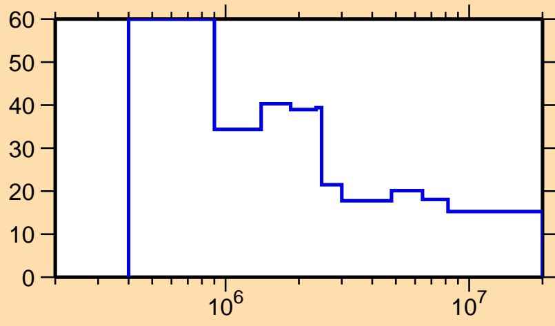
\Delta\sigma/\sigma vs. E for ^{230}\text{Ac}(n,\text{nonel.})
