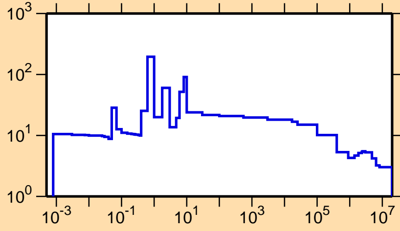
\sigma vs. E for ^{230}\text{Ac}(n,\text{el.})
