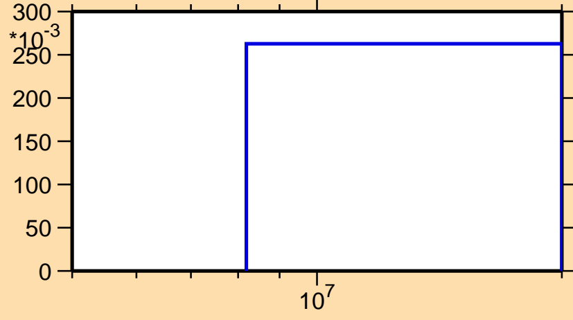
\sigma vs. E for ^{230}\text{Ac}(n,3n)
