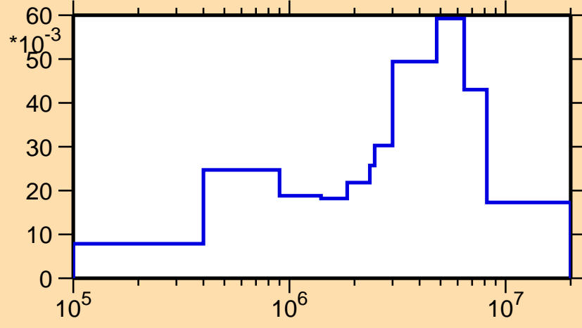
\sigma vs. E for ^{230}\text{Ac}(n,n_4)
