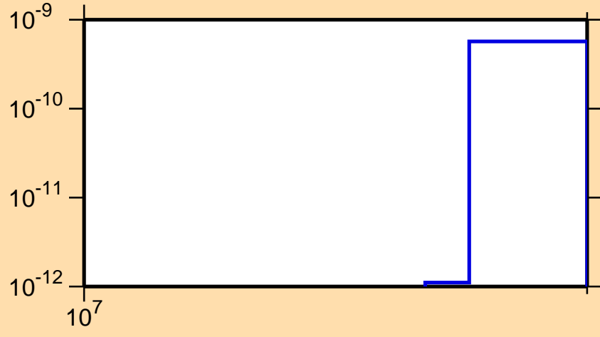
\sigma vs. E for ^{231}\text{Ac}(n,3n\alpha)
