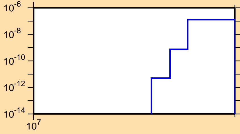
\sigma vs. E for ^{231}\text{Ac}(n,2np)
