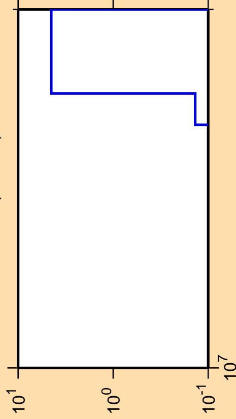
\Delta\sigma/\sigma vs. E for ^{231}\text{Ac}(n,\text{He}3)
