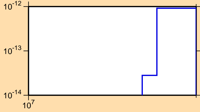
\sigma vs. E for ^{231}\text{Ac}(n,\text{He}3)
