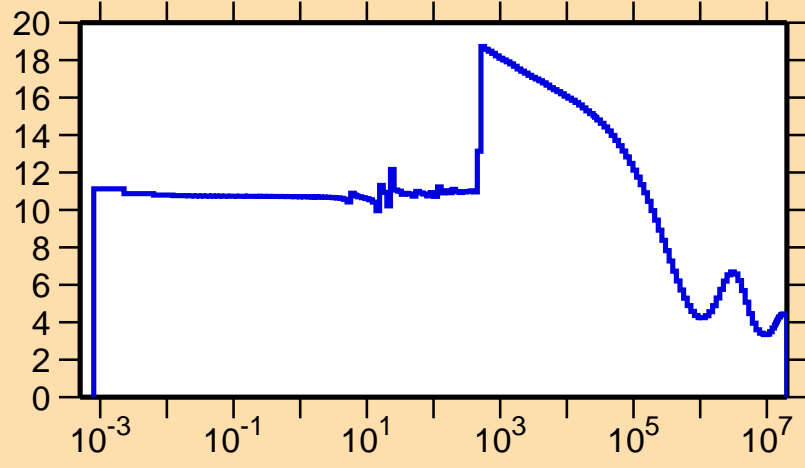
\sigma vs. E for ^{231}\text{Ac}(n,\text{el.})
