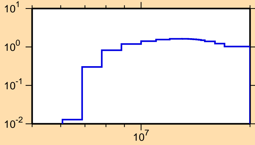
\sigma vs. E for ^{231}\text{Ac}(n,2n)
