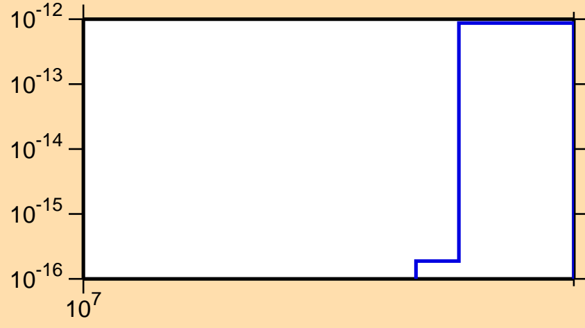
\sigma vs. E for ^{231}\text{Ac} (mt 11)
