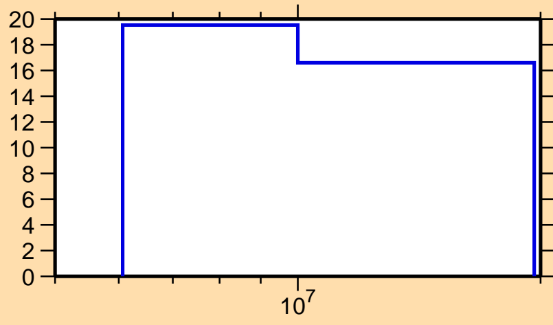
\Delta\sigma/\sigma vs. E for ^{231}\text{Ac}(n,\text{nonel.})
