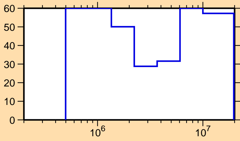
\Delta\sigma/\sigma vs. E for ^{231}\text{Ac}(n,n\text{cont.})
