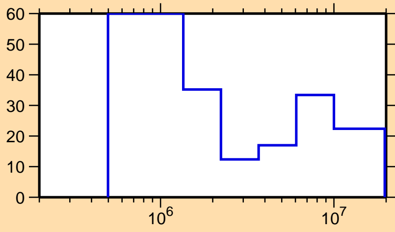
\Delta\sigma/\sigma vs. E for ^{231}\text{Ac}(n,\text{el.})
