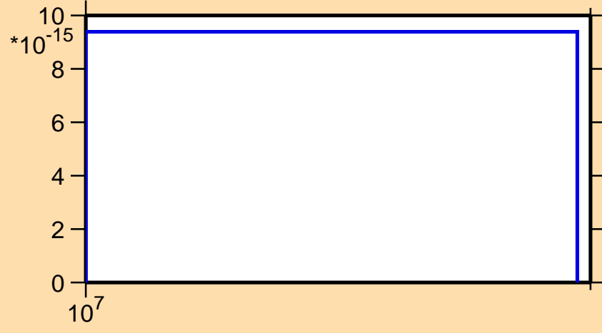
\sigma vs. E for ^{231}\text{Ac}(n,\text{He3})
