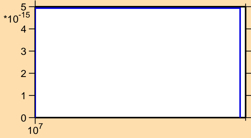
\sigma vs. E for ^{231}\text{Ac} (mt 11)
