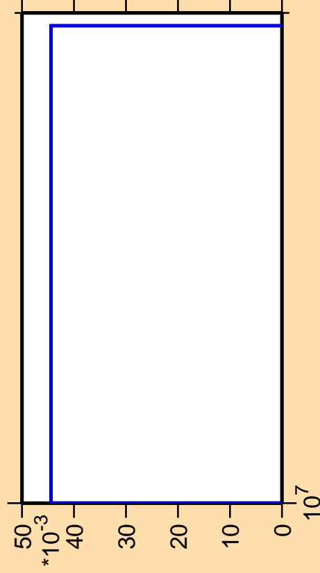
\Delta\sigma/\sigma vs. E for ^{231}\text{Ac}(n,\text{He3})
