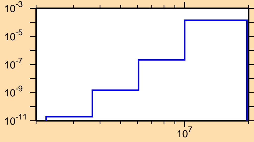
\sigma vs. E for ^{231}\text{Ac}(n,\alpha)
