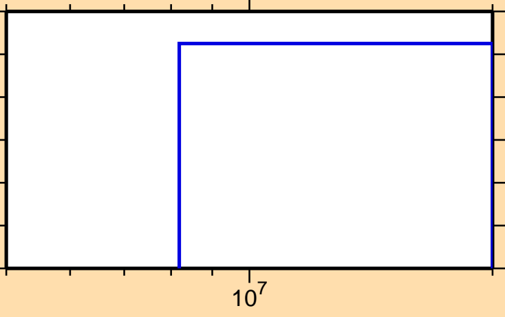
\sigma vs. E for ^{231}\text{Ac}(n,\text{nd})
