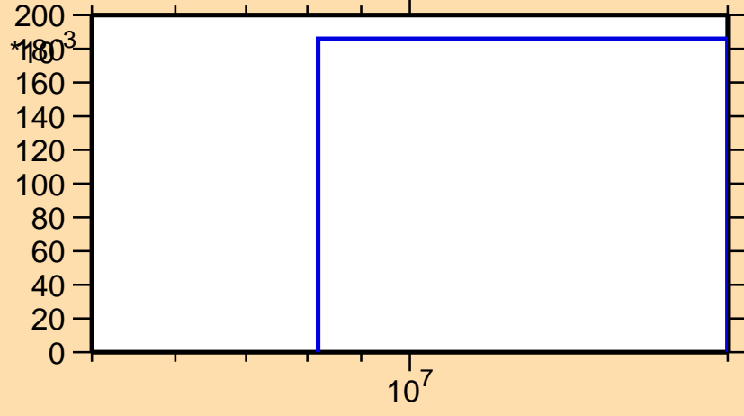
\sigma vs. E for ^{231}\text{Ac}(n,3n)
