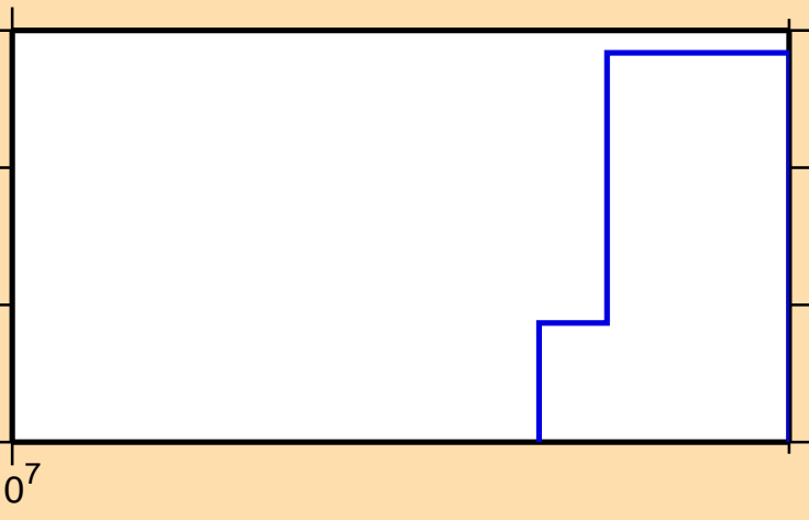
\sigma vs. E for ^{232}\text{Ac}(n,\text{He3})
