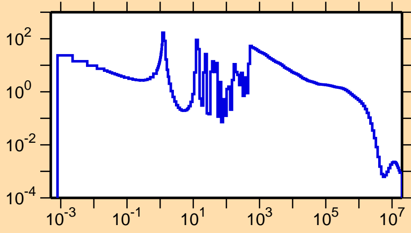
\sigma vs. E for ^{233}\text{Ac}(n,\gamma)
