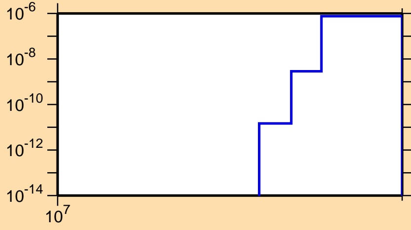
\sigma vs. E for ^{233}\text{Ac}(n,2np)
