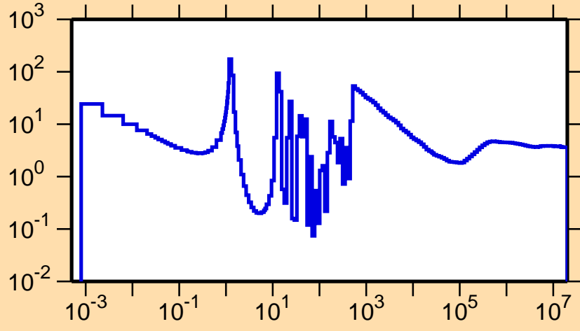
\sigma vs. E for ^{233}\text{Ac}(n,\text{nonel.})
