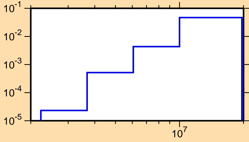
\sigma vs. E for ^{233}\text{Ac}(n,\alpha)
