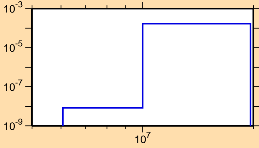
\sigma vs. E for ^{233}\text{Ac}(n,n\alpha)
