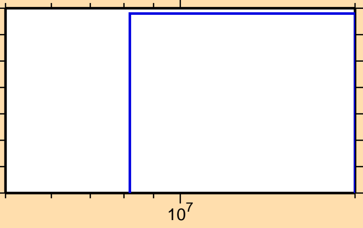
\sigma vs. E for ^{233}\text{Ac}(\text{mt 11})
