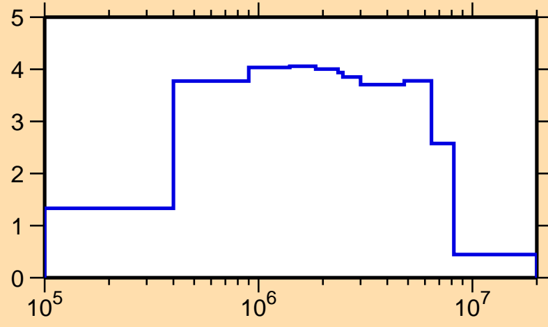
\sigma vs. E for ^{233}\text{Ac}(n,\text{inel.})
