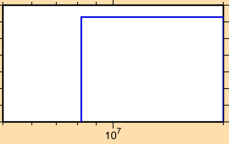
\sigma vs. E for ^{233}\text{Ac}(n,2np)
