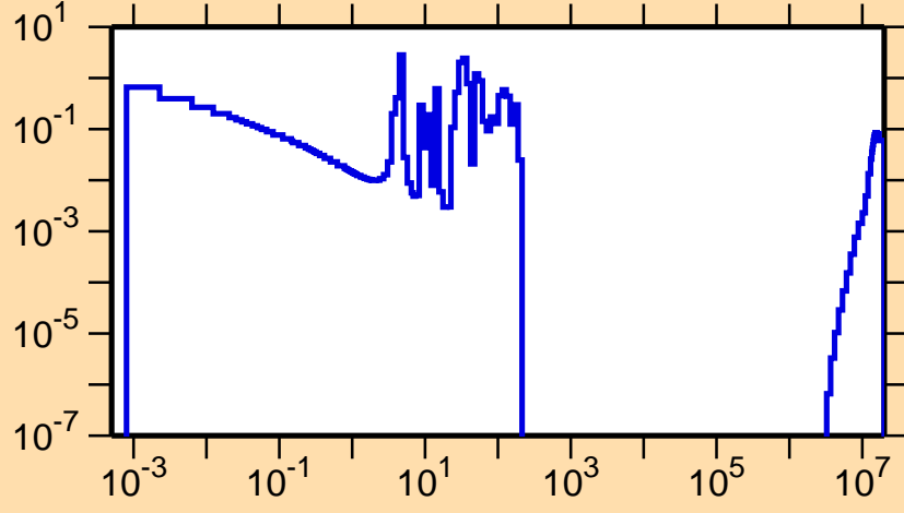
\sigma vs. E for ^{235}\text{Ac}(n,f)
