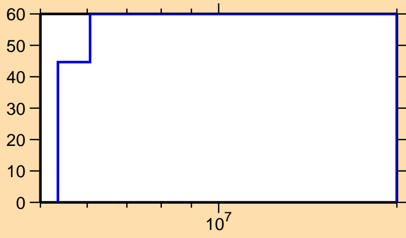
\Delta\sigma/\sigma vs. E for ^{235}\text{Ac}(n,\text{inel.})
