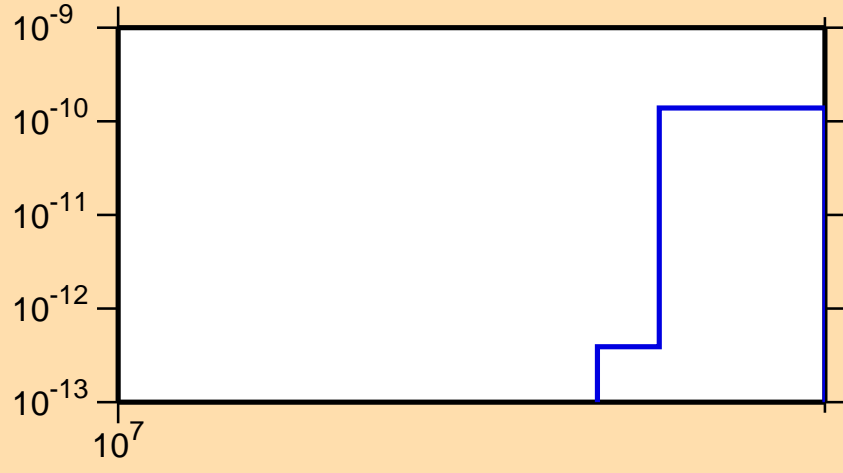
\sigma vs. E for ^{235}\text{Ac}(n,3n\alpha)
