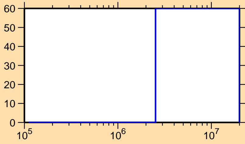
\Delta\sigma/\sigma vs. E for ^{235}\text{Ac}(n,f)
