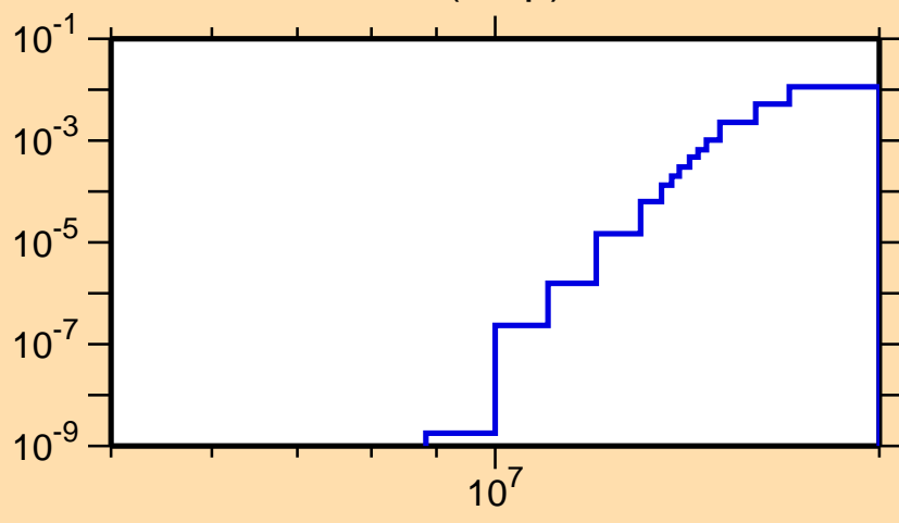
\sigma vs. E for ^{235}\text{Ac}(n,np)
