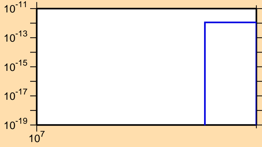
\sigma vs. E for ^{235}\text{Ac}(\text{mt } 11)
