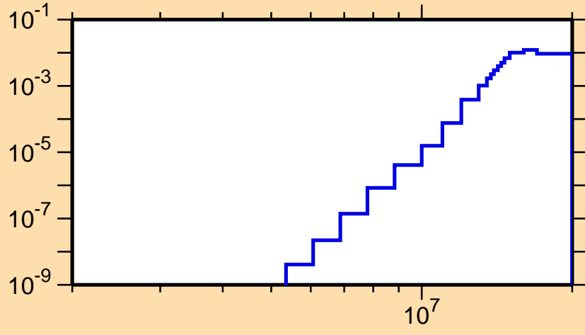
\sigma vs. E for ^{235}\text{Ac}(n,\alpha)
