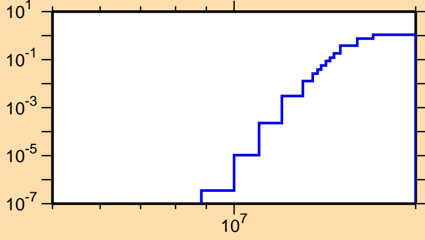
\sigma vs. E for ^{235}\text{Ac}(n,t)
