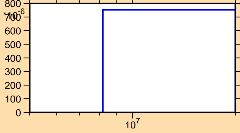
\sigma vs. E for ^{235}\text{Ac}(n,np)
