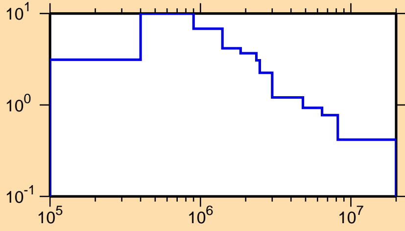
\sigma vs. E for ^{235}\text{Ac}(n,n_1)
