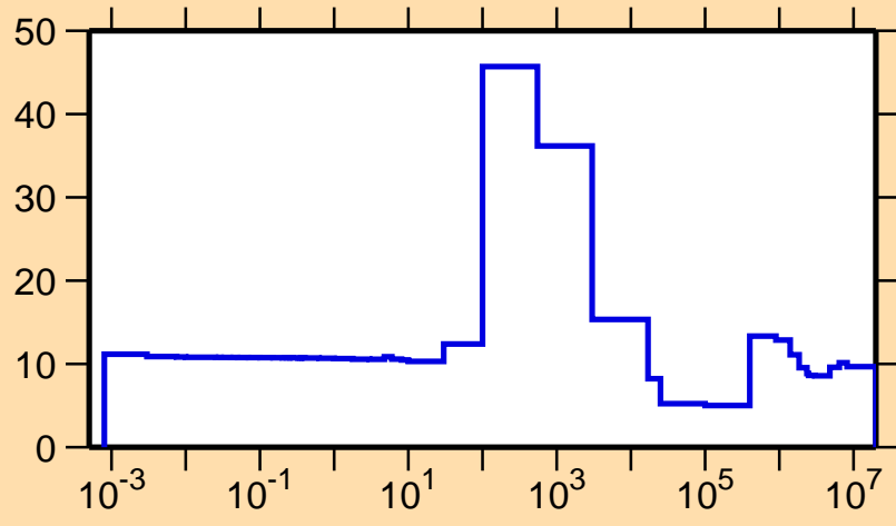
\sigma vs. E for ^{235}\text{Ac}(n,\text{el.})
