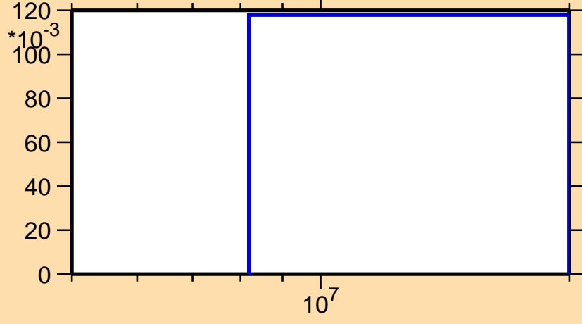
\sigma vs. E for ^{235}\text{Ac}(n,t)
