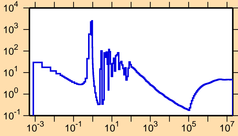
\sigma vs. E for ^{236}\text{Ac}(n,\text{nonel.})
