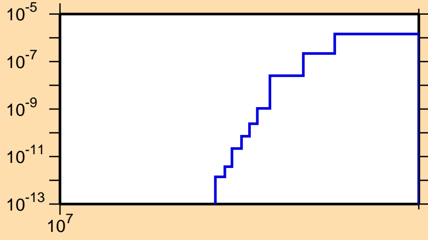
\sigma vs. E for ^{236}\text{Ac}(n,2np)
