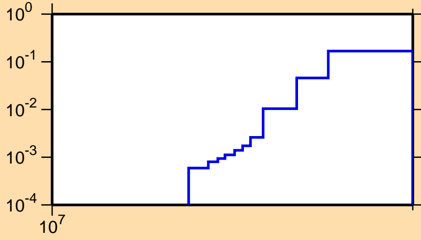
\sigma vs. E for ^{236}\text{Ac}(n,2n\alpha)
