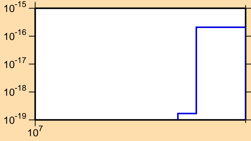
\sigma vs. E for ^{236}\text{Ac}(\text{mt } 11)
