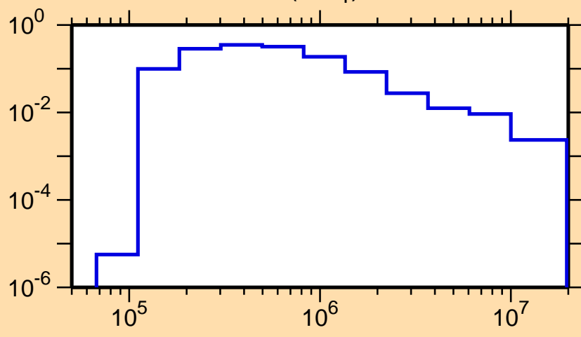
\sigma vs. E for ^{236}\text{Ac}(n,n_1)
