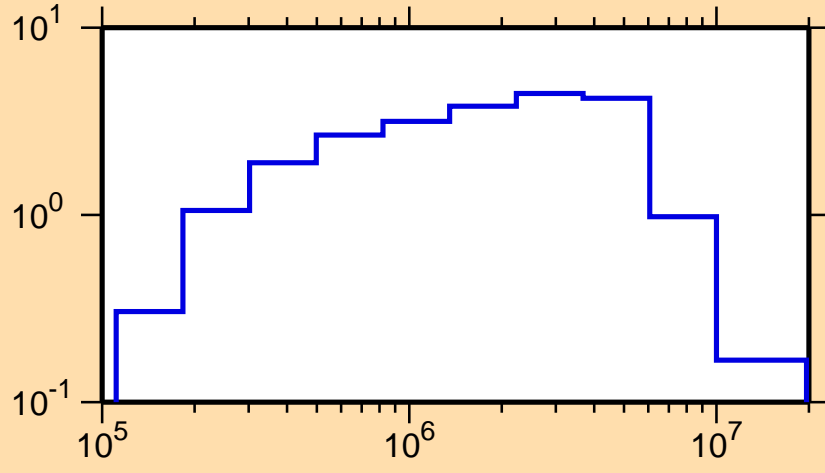
\sigma vs. E for ^{236}\text{Ac}(n,\text{inel.})
