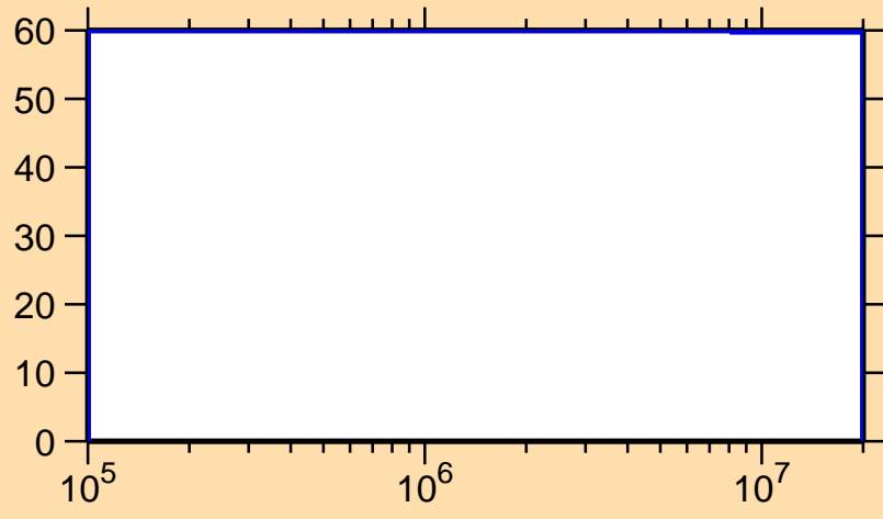
\Delta\sigma/\sigma vs. E for ^{236}\text{Ac}(n,\text{nonel.})
