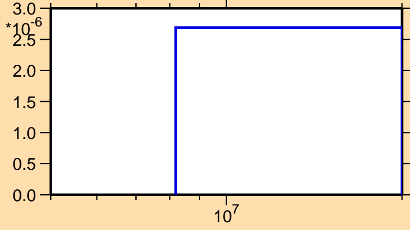
\sigma vs. E for ^{236}\text{Ac}(n,d)
