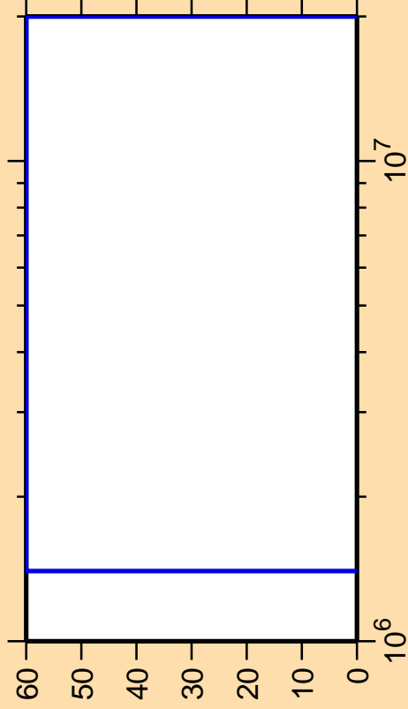
\Delta\sigma/\sigma vs. E for ^{236}\text{Ac}(n,n_1)
