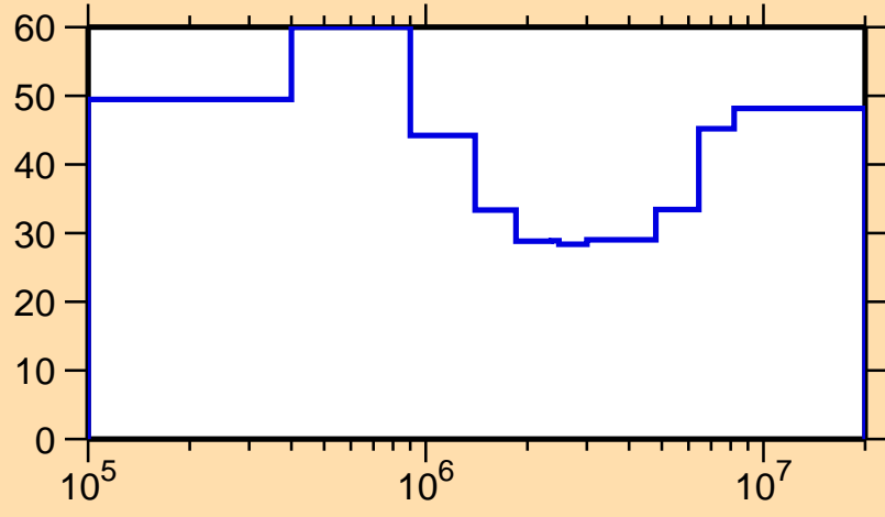
\Delta\sigma/\sigma vs. E for ^{236}\text{Ac}(n,\text{tot.})
