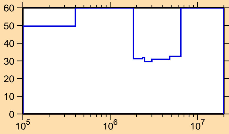
\Delta\sigma/\sigma vs. E for ^{236}\text{Ac}(n,\text{el.})
