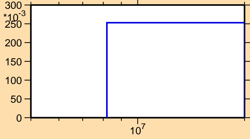
\sigma vs. E for ^{236}\text{Ac}(n,3n)
