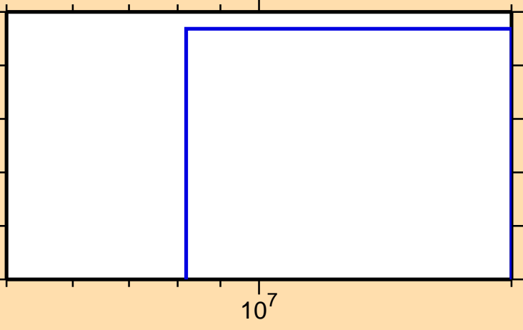
\sigma vs. E for ^{236}\text{Ac}(n,2np)
