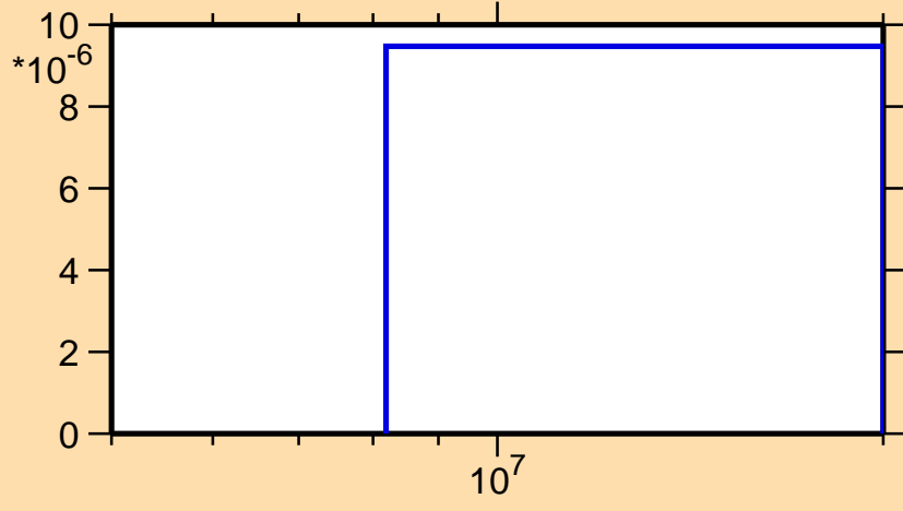
\sigma vs. E for ^{236}\text{Ac}(n,np)
