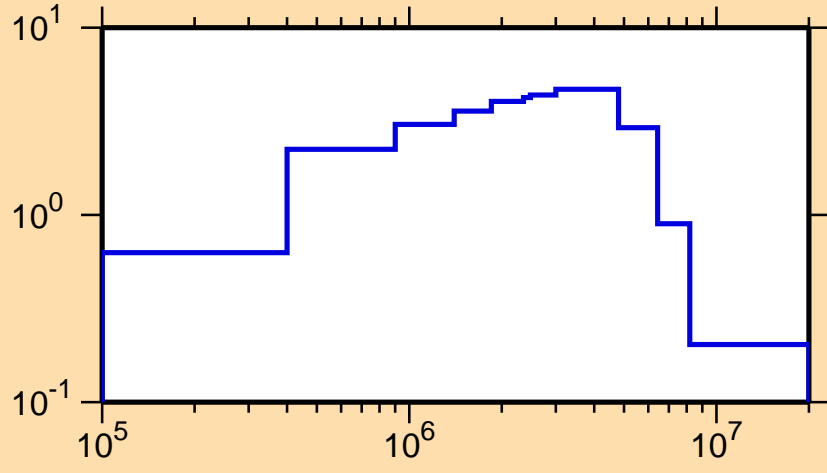
\sigma vs. E for ^{236}\text{Ac}(n,n\text{cont.})
