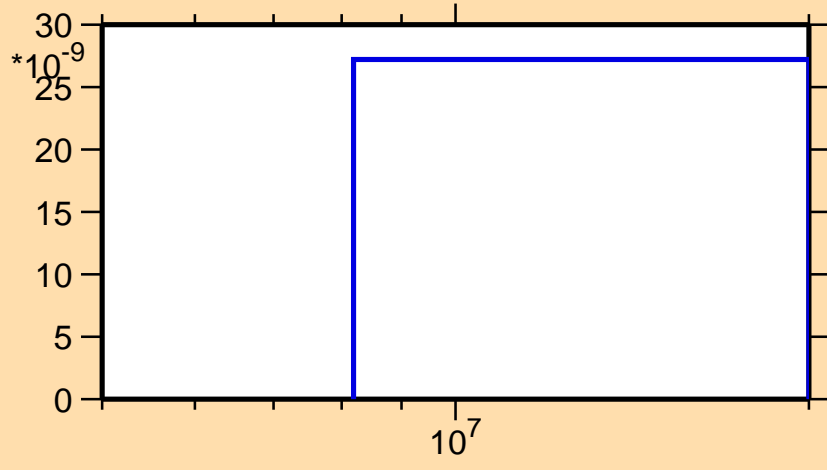
\sigma vs. E for ^{236}\text{Ac}(n,\text{nd})
