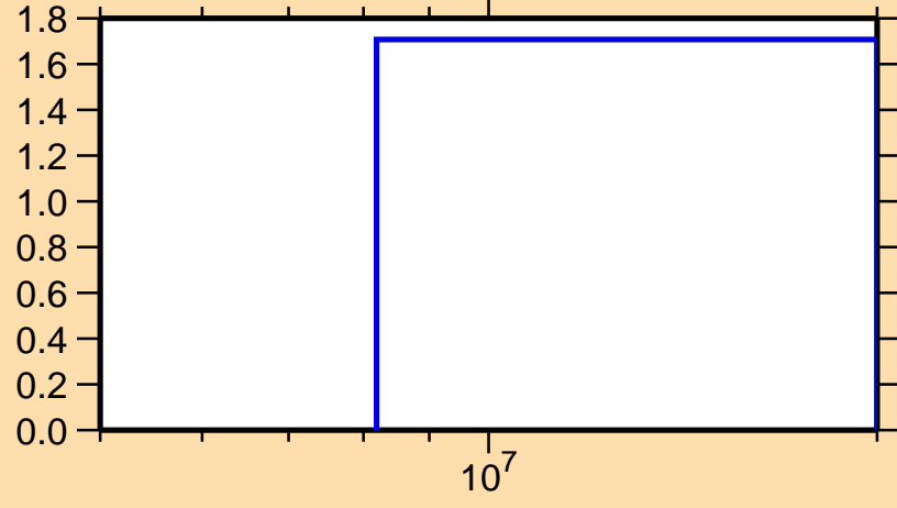
\sigma vs. E for ^{236}\text{Ac}(n,n\alpha)
