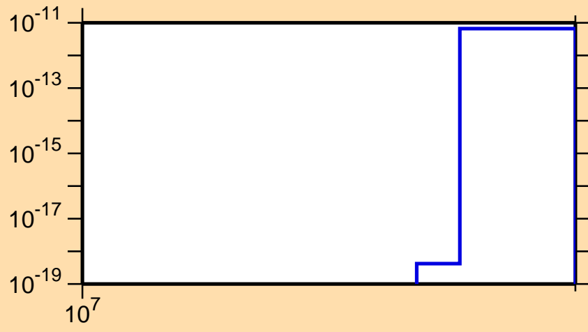
\sigma vs. E for ^{237}\text{Ac}(\text{mt } 11)
