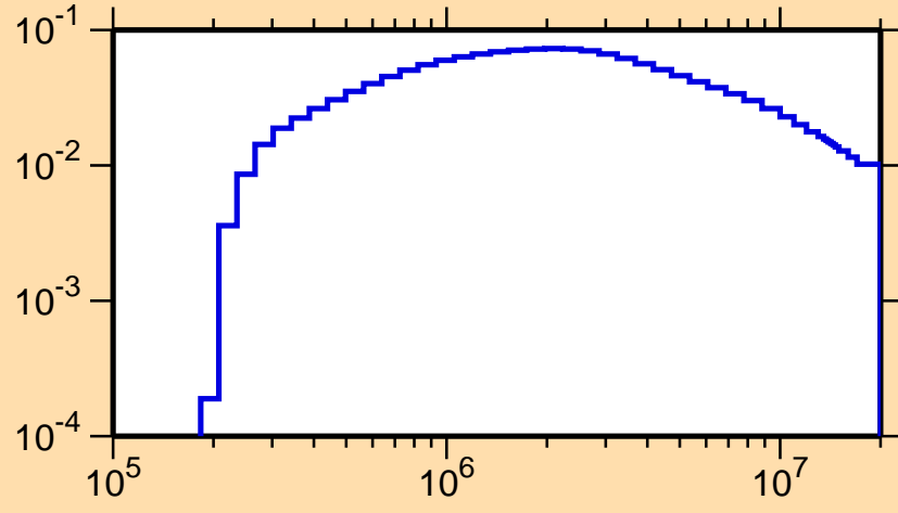
\sigma vs. E for ^{237}\text{Ac}(n,n_1)
