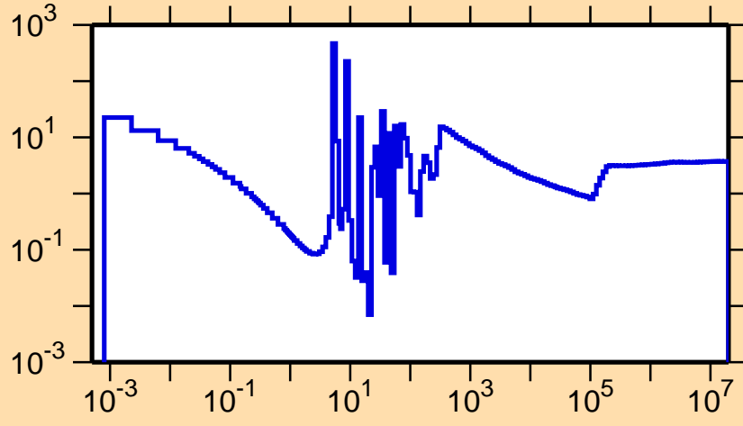
\sigma vs. E for ^{237}\text{Ac}(n,\text{nonel.})
