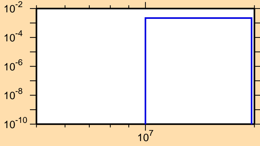
\sigma vs. E for ^{237}\text{Ac}(n,n\alpha)
