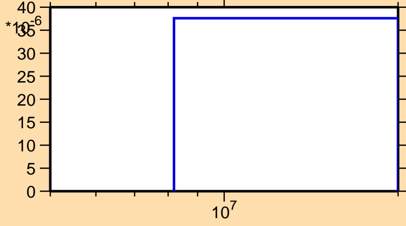
\sigma vs. E for ^{237}\text{Ac}(n,d)
