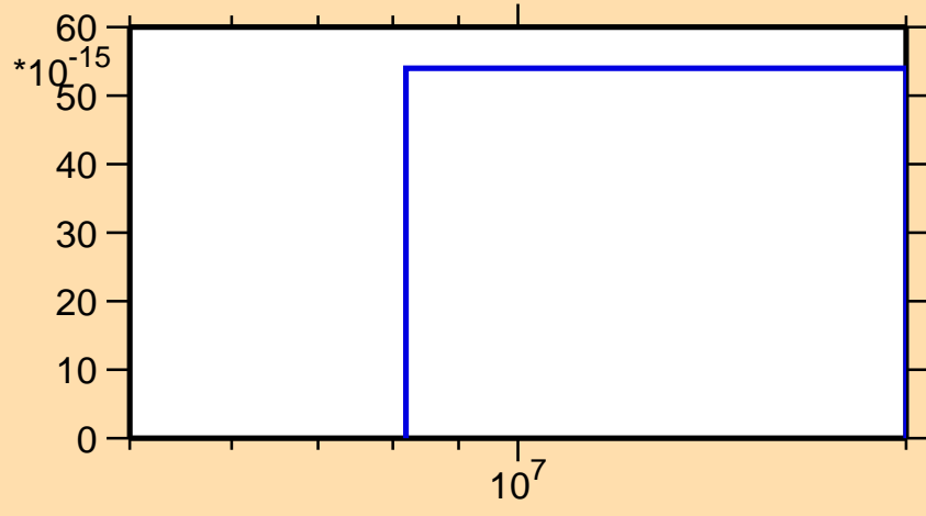
\sigma vs. E for ^{237}\text{Ac} (mt 11)
