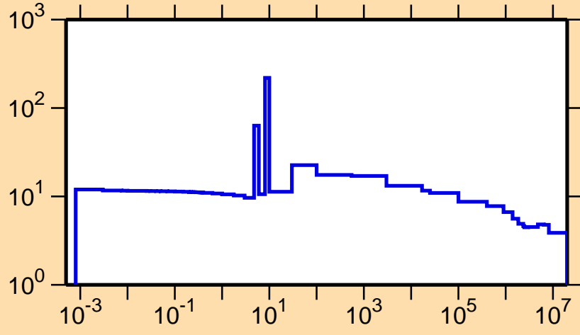
\sigma vs. E for ^{237}\text{Ac}(n,\text{el.})
