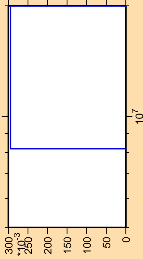
\Delta\sigma/\sigma vs. E for ^{237}\text{Ac} (mt 11)
