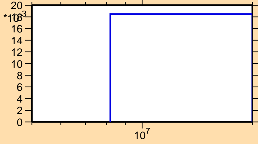
\sigma vs. E for ^{237}\text{Ac}(n,3n)
