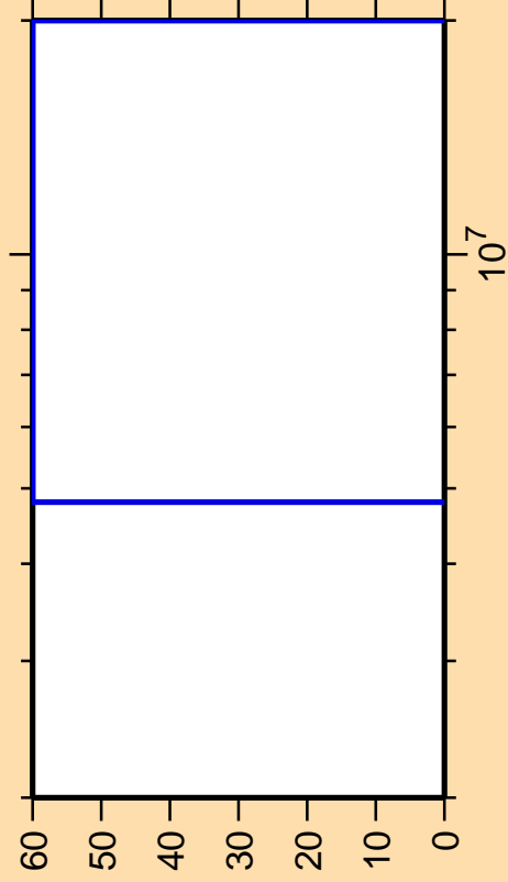
\Delta\sigma/\sigma vs. E for ^{237}\text{Ac}(n,n_1)
