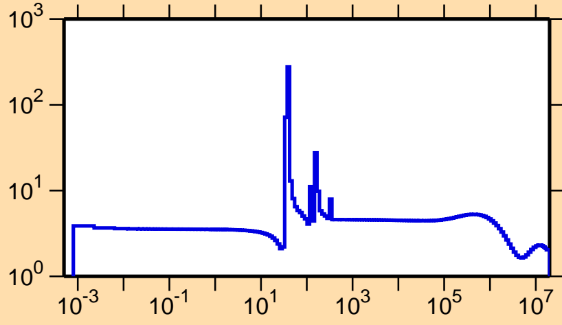
\sigma vs. E for ^{96}\text{Ag}(n,\text{el.})
