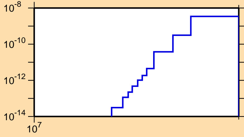
\sigma vs. E for ^{96}\text{Ag}(\text{mt117})
