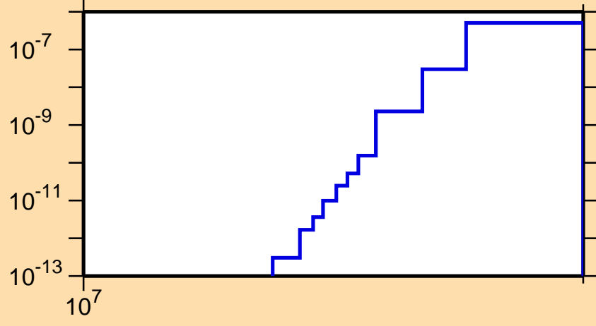
\sigma vs. E for ^{96}\text{Ag} (mt 45)
