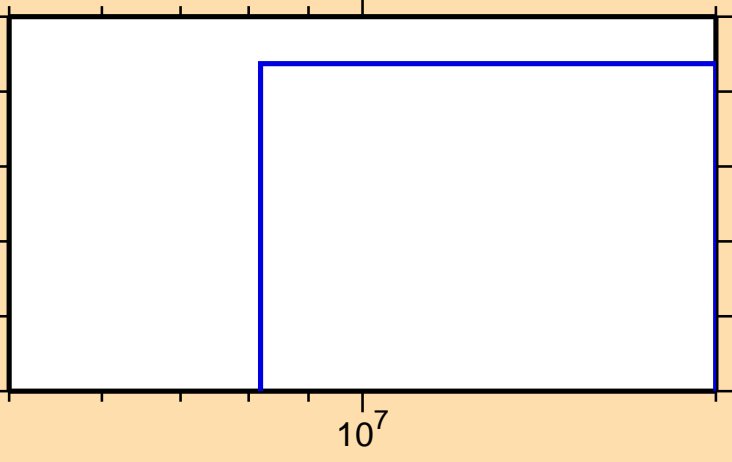
\sigma vs. E for ^{96}\text{Ag}(n,\text{nd})
