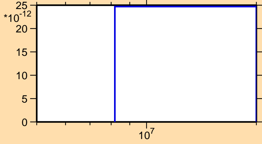
\sigma vs. E for ^{96}\text{Ag} (mt 34)
