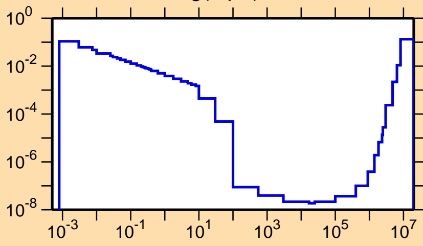
\sigma vs. E for ^{96}\text{Ag}(n,p\alpha)
