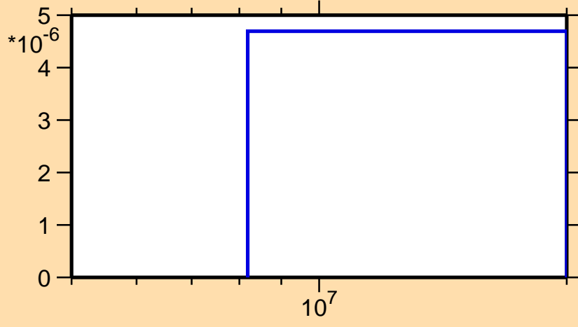
\sigma vs. E for ^{96}\text{Ag}(n,n\alpha)
