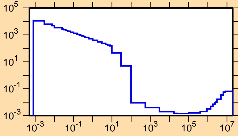
\sigma vs. E for ^{96}\text{Ag}(n,\alpha)
