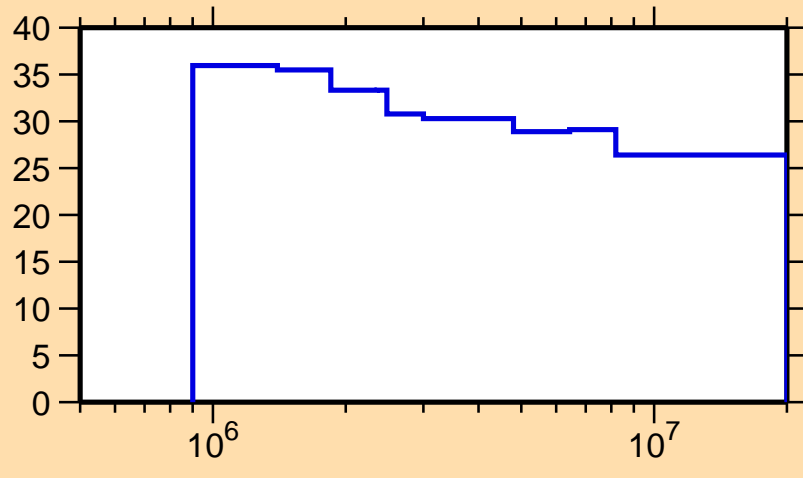
\Delta\sigma/\sigma vs. E for ^{96}\text{Ag}(n,ncont.)
