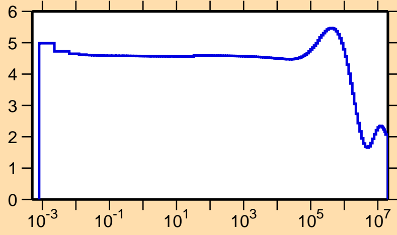
\sigma vs. E for ^{98}\text{Ag}(n,\text{el.})
