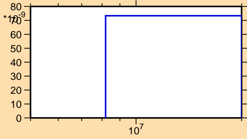
\sigma vs. E for ^{98}\text{Ag}(\text{mt } 45)
