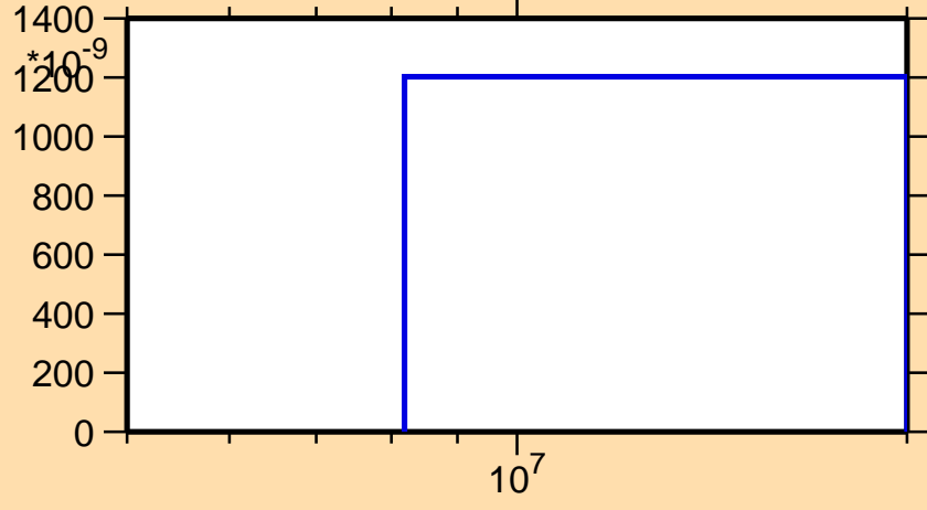
\sigma vs. E for ^{98}\text{Ag}(n,pt)
