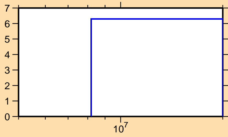
\Delta\sigma/\sigma vs. E for ^{98}\text{Ag}(n,\text{el.})
