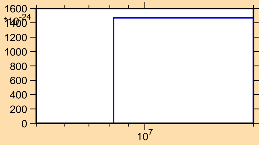
\sigma vs. E for ^{98}\text{Ag}(n,nt)
