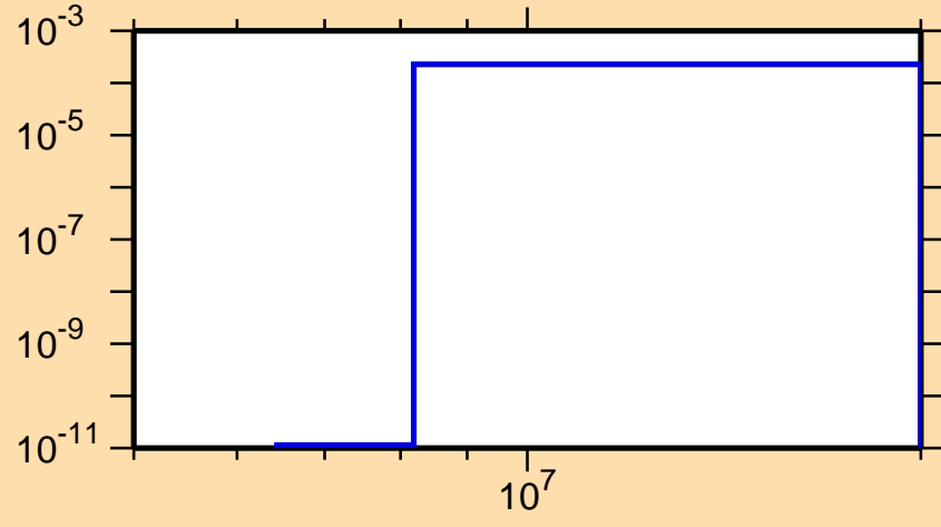
\sigma vs. E for ^{98}\text{Ag}(n,n\alpha)
