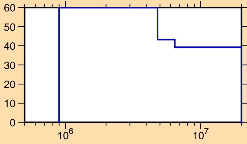
\Delta\sigma/\sigma vs. E for ^{98}\text{Ag}(n,n\text{cont.})
