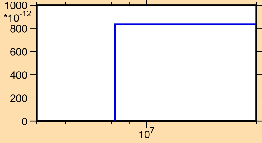
\sigma vs. E for ^{98}\text{Ag} (mt 34)
