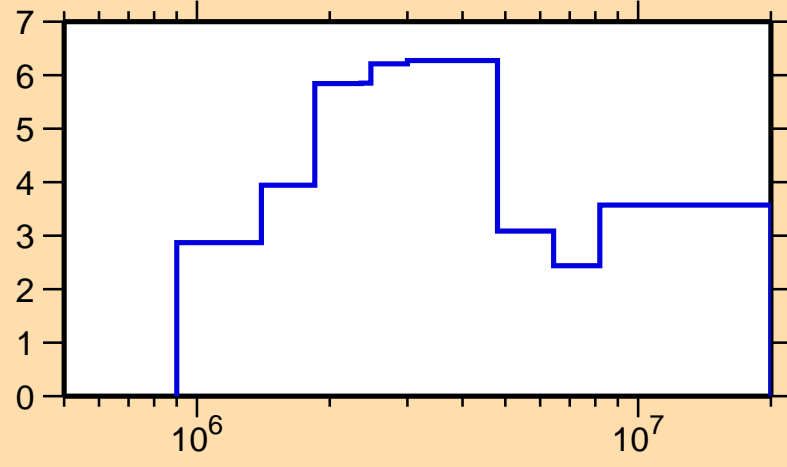
\Delta\sigma/\sigma vs. E for ^{98}\text{Ag}(n,\text{tot.})
