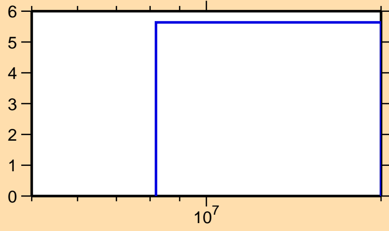
\Delta\sigma/\sigma vs. E for ^{98}\text{Ag}(n,\text{nonel.})
