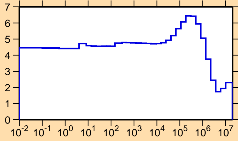
\sigma vs. E for ^{99}\text{Ag}(n,\text{el.})
