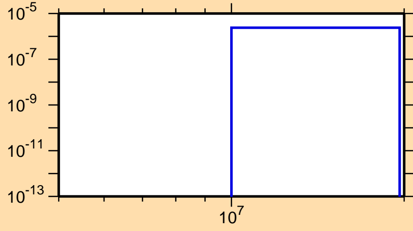
\sigma vs. E for ^{99}\text{Ag} (mt 45)
