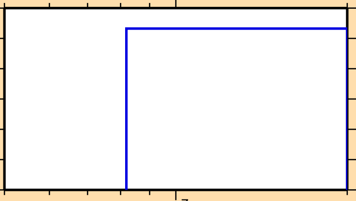
\sigma vs. E for ^{99}\text{Ag}(n,\text{pt})
