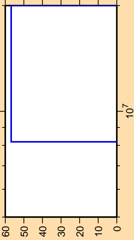
\Delta\sigma/\sigma vs. E for ^{99}\text{Ag}(n,2n)
