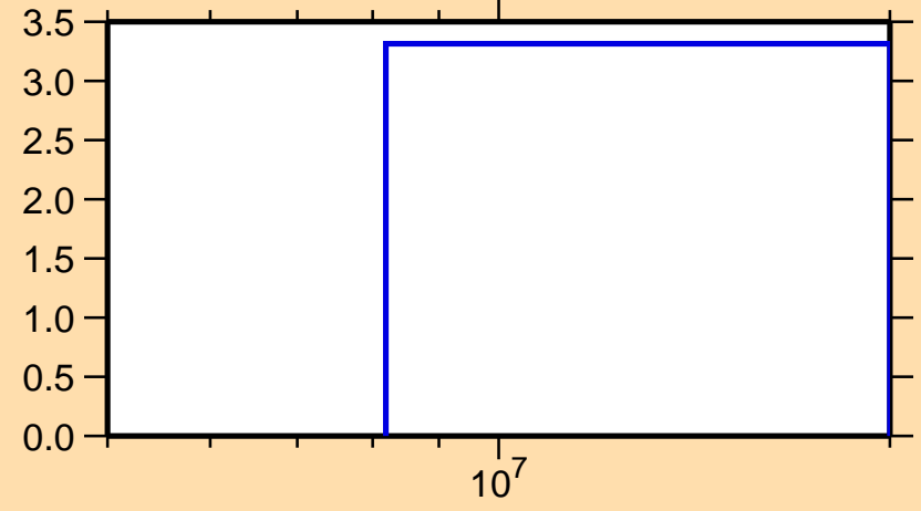
\Delta\sigma/\sigma vs. E for ^{99}\text{Ag}(n,\text{tot.})
