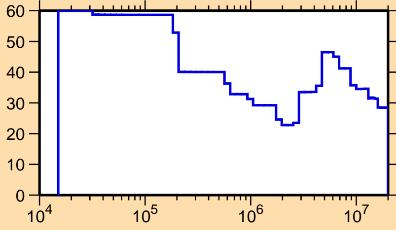
\Delta\sigma/\sigma vs. E for ^{100}\text{Ag}(n,n_1)
