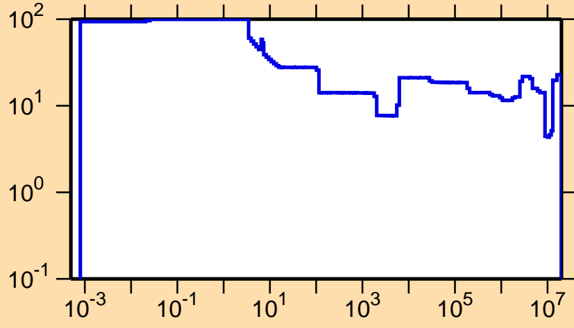
\Delta\sigma/\sigma vs. E for ^{100}\text{Ag}(n,p)
