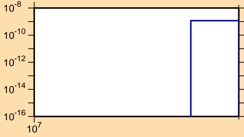
\sigma vs. E for ^{100}\text{Ag}(n,nt)
