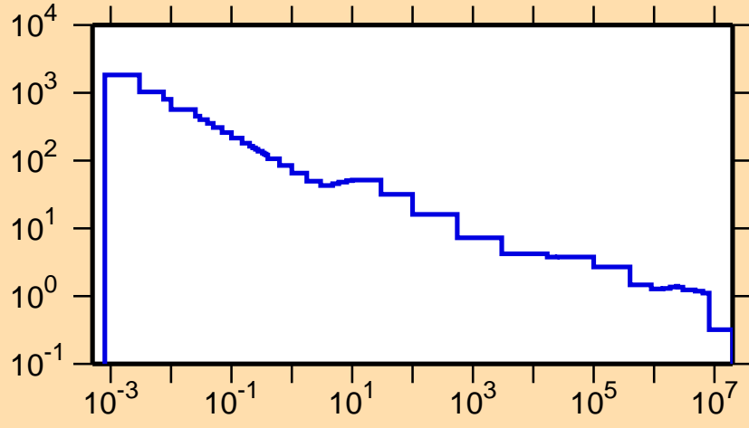
\sigma vs. E for ^{100}\text{Ag}(n,p)
