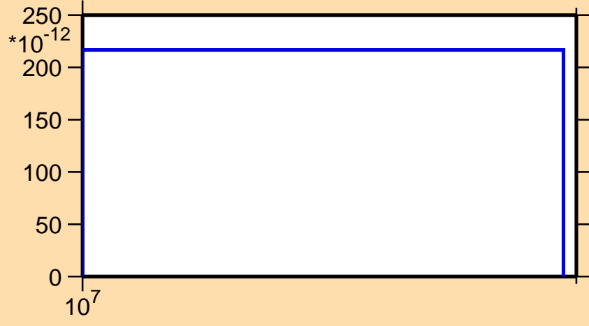
\sigma vs. E for ^{100}\text{Ag} (mt 34)
