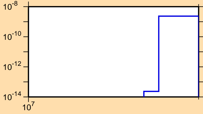
\sigma vs. E for ^{101}\text{Ag}(n,\text{pt})
