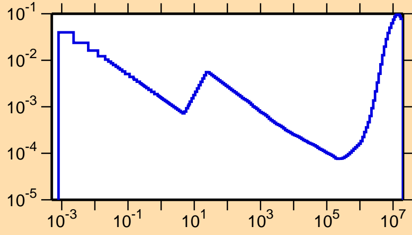
\sigma vs. E for ^{101}\text{Ag}(n,\alpha)
