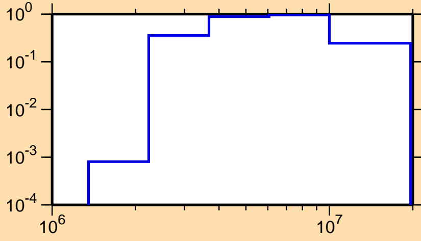
\sigma vs. E for ^{101}\text{Ag}(n,n\text{cont.})
