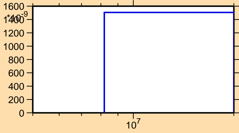
\sigma vs. E for ^{101}\text{Ag}(n,\text{pd})
