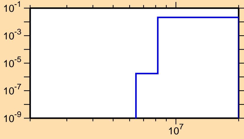
\sigma vs. E for ^{101}\text{Ag}(n,n\alpha)
